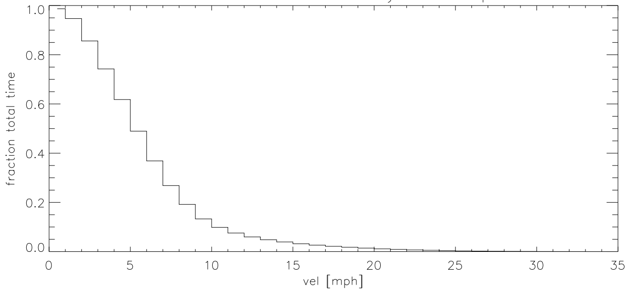
AUG10 Fraction of time wind velocity exceeds specified vel (blowup)
