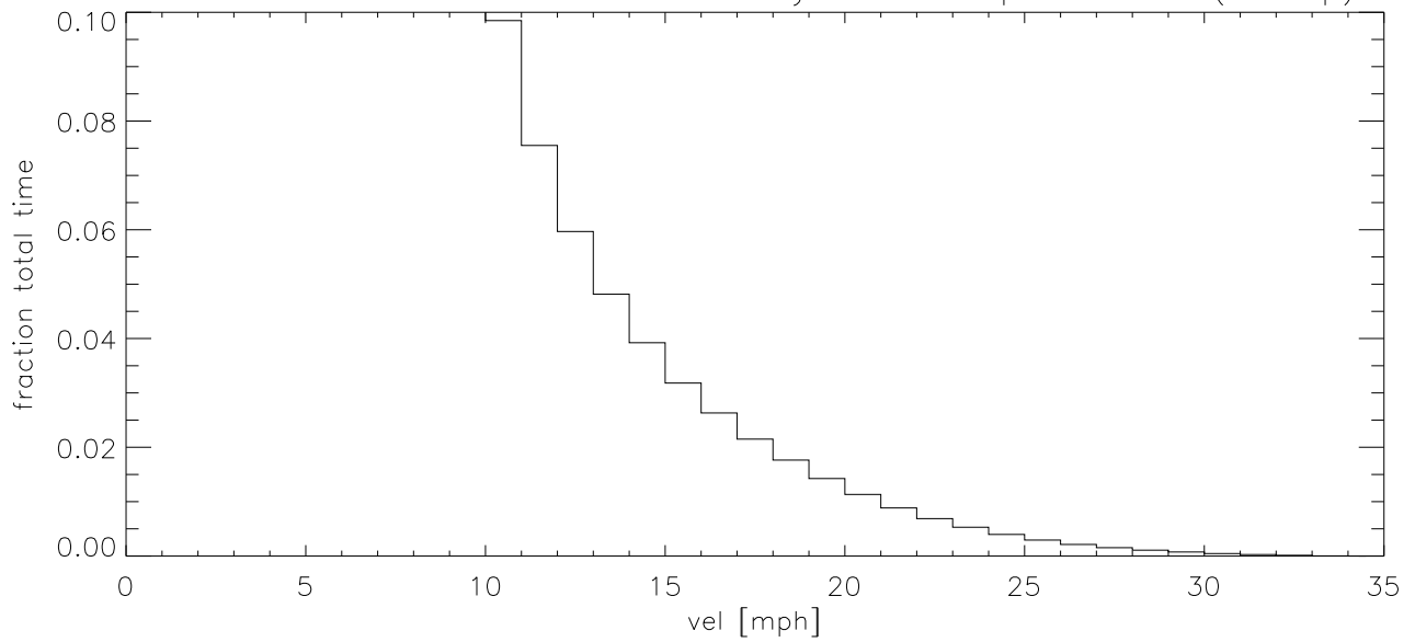
AUG10 Fraction of time wind velocity exceeds specified vel (blowup)
