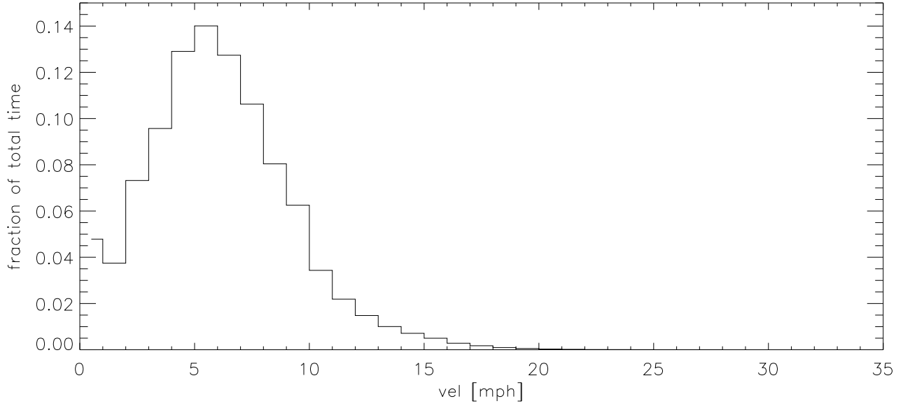
JUN10 Fraction of time wind velocity exceeds specified vel
