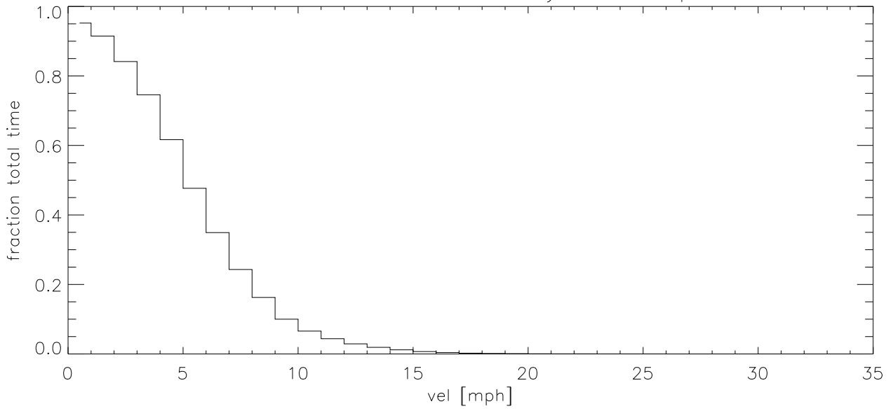
JUN10 Fraction of time wind velocity exceeds specified vel (blowup)
