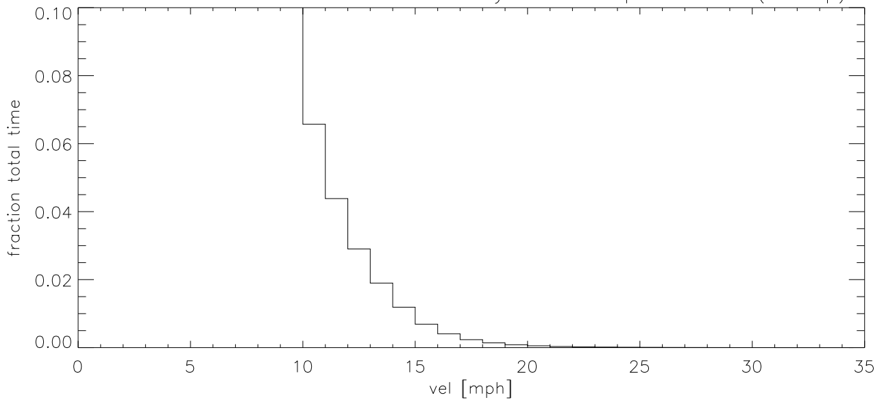
JUN10 Fraction of time wind velocity exceeds specified vel (blowup)
