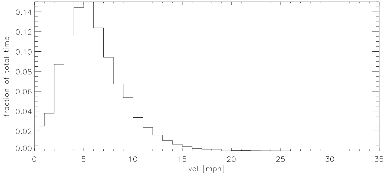
MAR10 Fraction of time wind velocity exceeds specified vel
