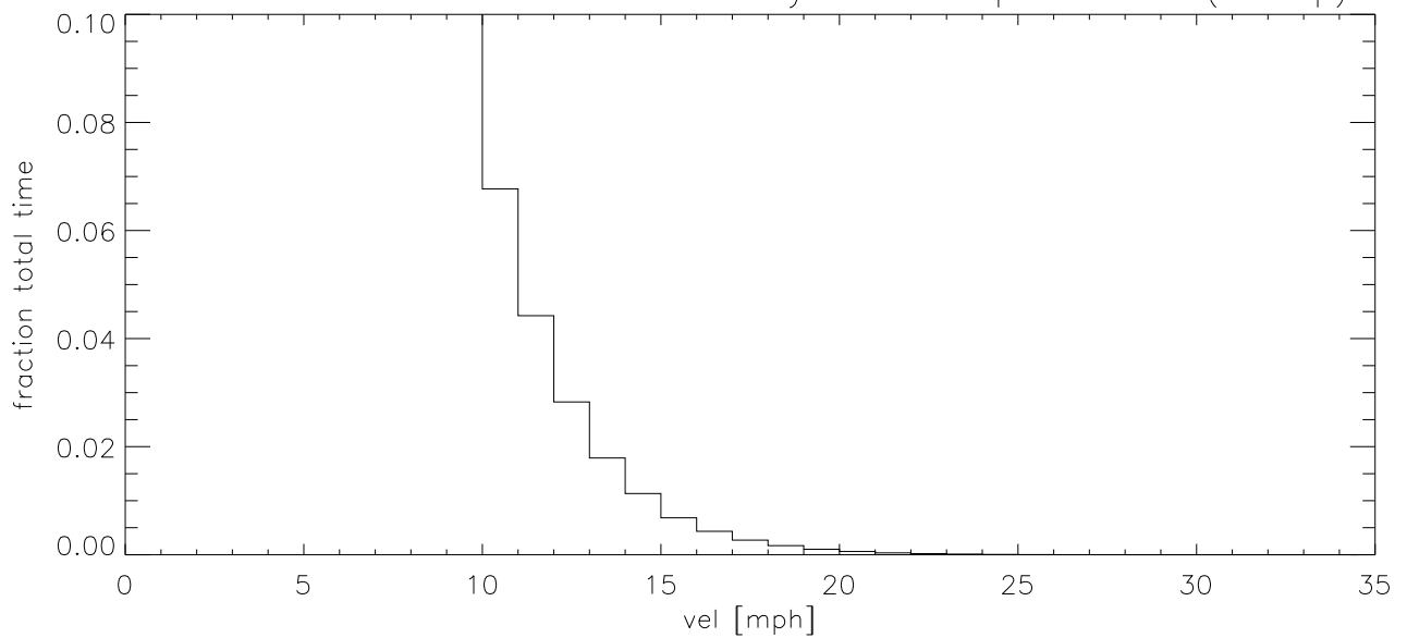
MAR10 Fraction of time wind velocity exceeds specified vel (blowup)
