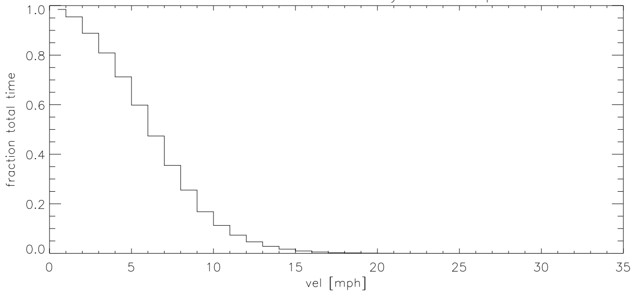
DEC09 Fraction of time wind velocity exceeds specified vel (blowup)
