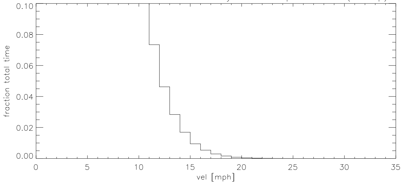
DEC09 Fraction of time wind velocity exceeds specified vel (blowup)
