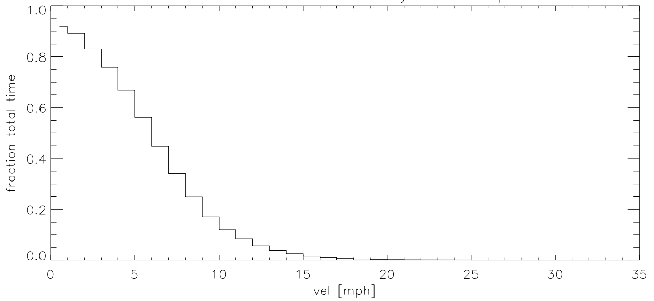
FEB09 Fraction of time wind velocity exceeds specified vel (blowup)
