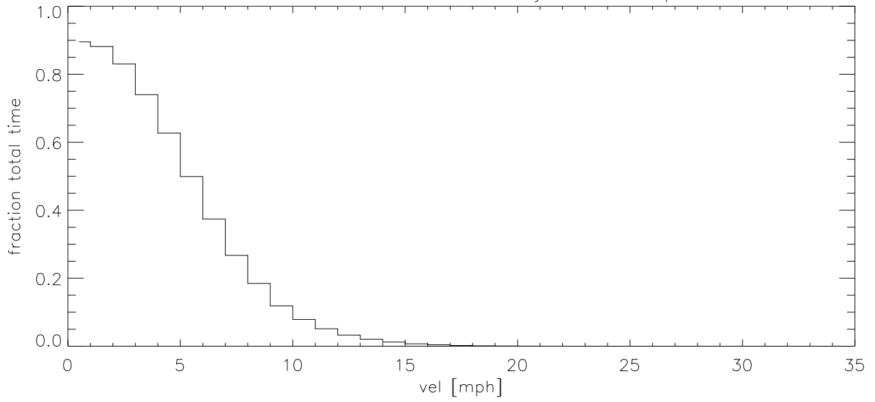
JAN09 Fraction of time wind velocity exceeds specified vel (blowup)
