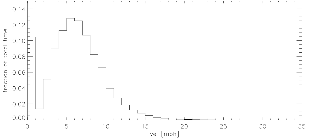
JAN09 Fraction of time wind velocity exceeds specified vel
