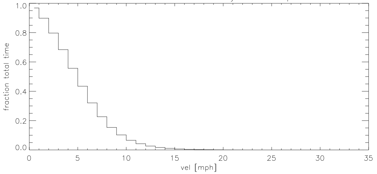
FEB07 Fraction of time wind velocity exceeds specified vel (blowup)
