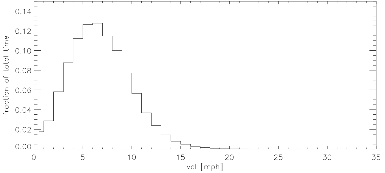
MAY04 Fraction of time wind velocity exceeds specified vel
