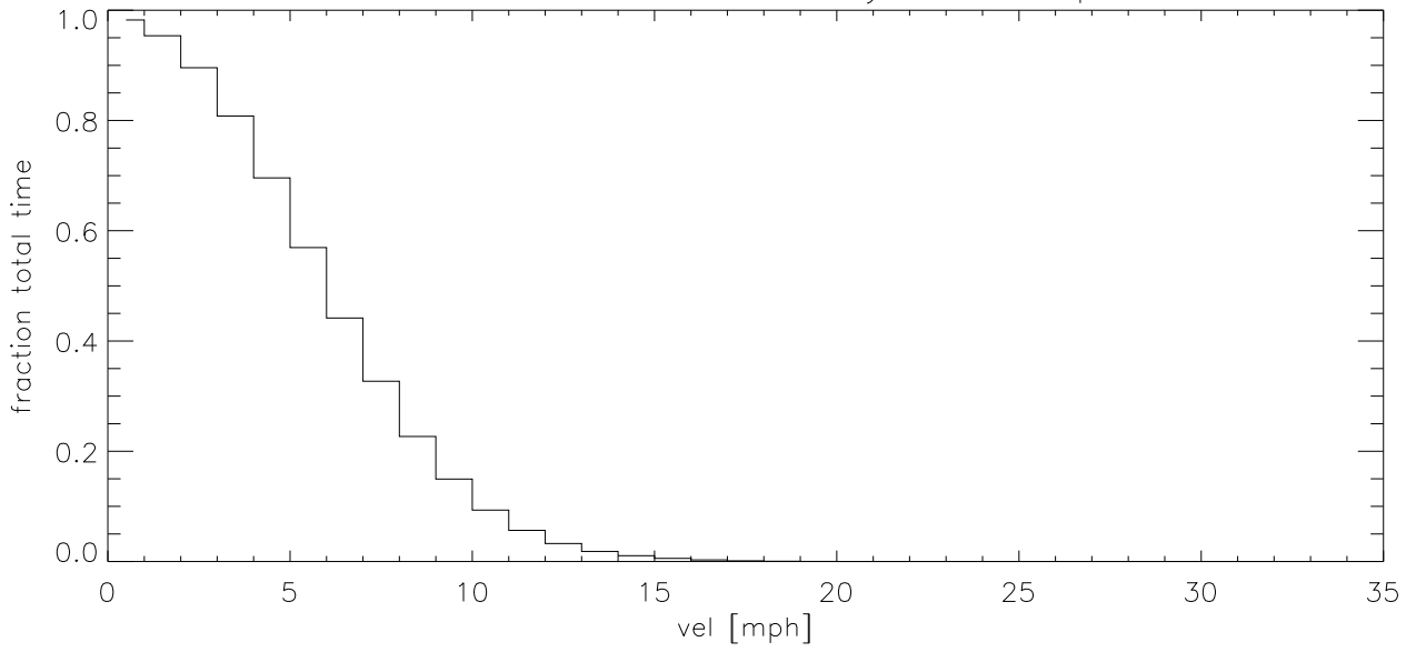
MAY04 Fraction of time wind velocity exceeds specified vel (blowup)
