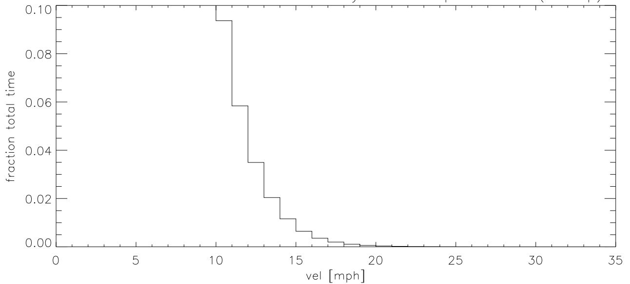
FEB04 Fraction of time wind velocity exceeds specified vel (blowup)
