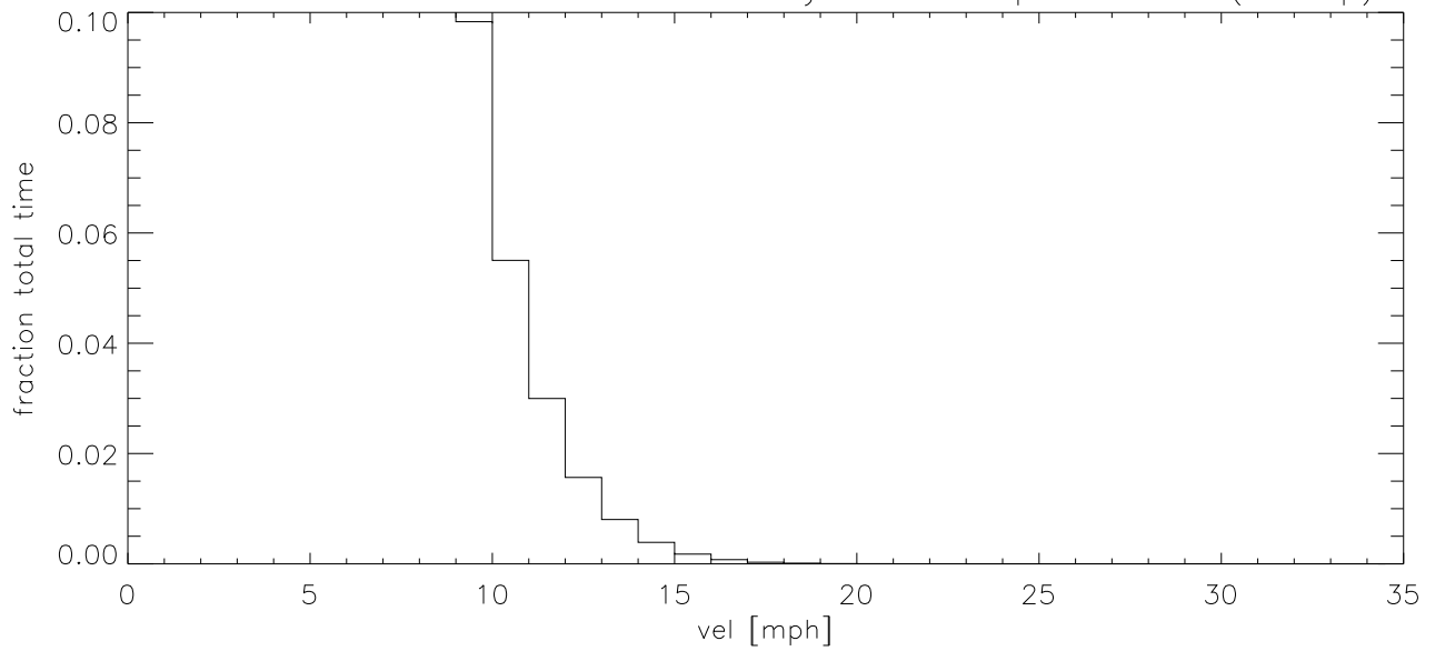
DEC02 Fraction of time wind velocity exceeds specified vel (blowup)
