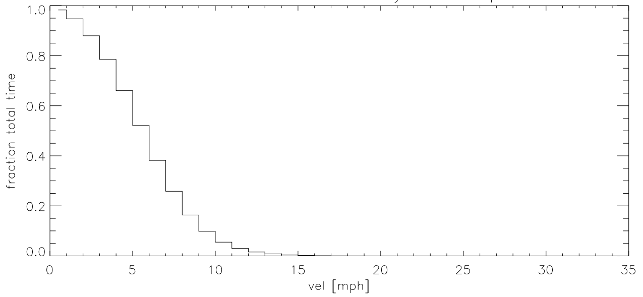
DEC02 Fraction of time wind velocity exceeds specified vel (blowup)
