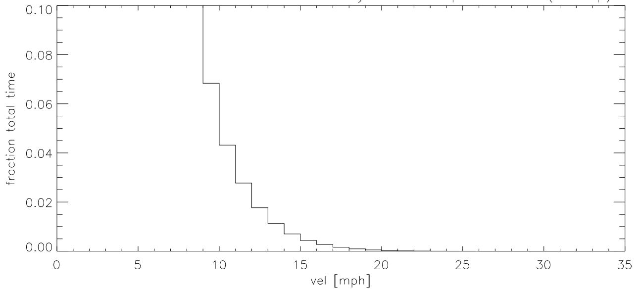
SEP02 Fraction of time wind velocity exceeds specified vel (blowup)
