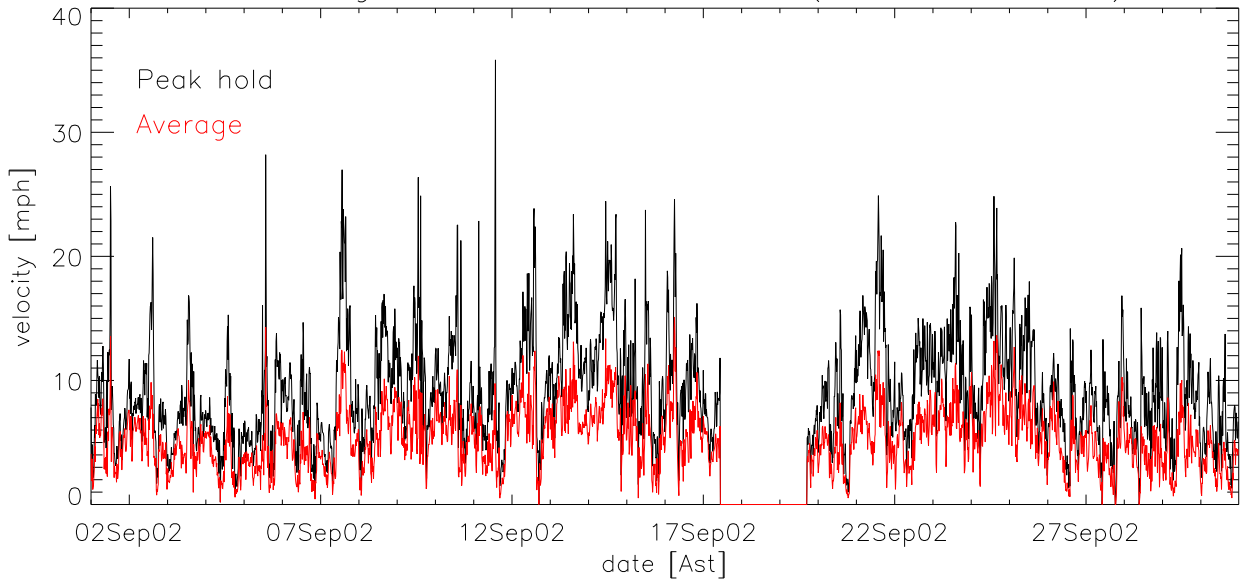
SEP02 Average, median velocity by hour of day
