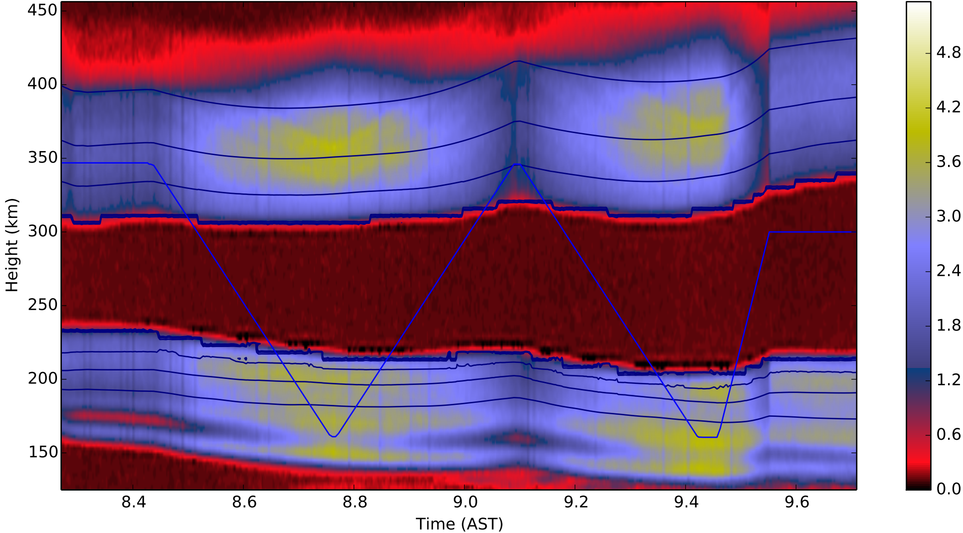
Plasma Line Power on 20150219
