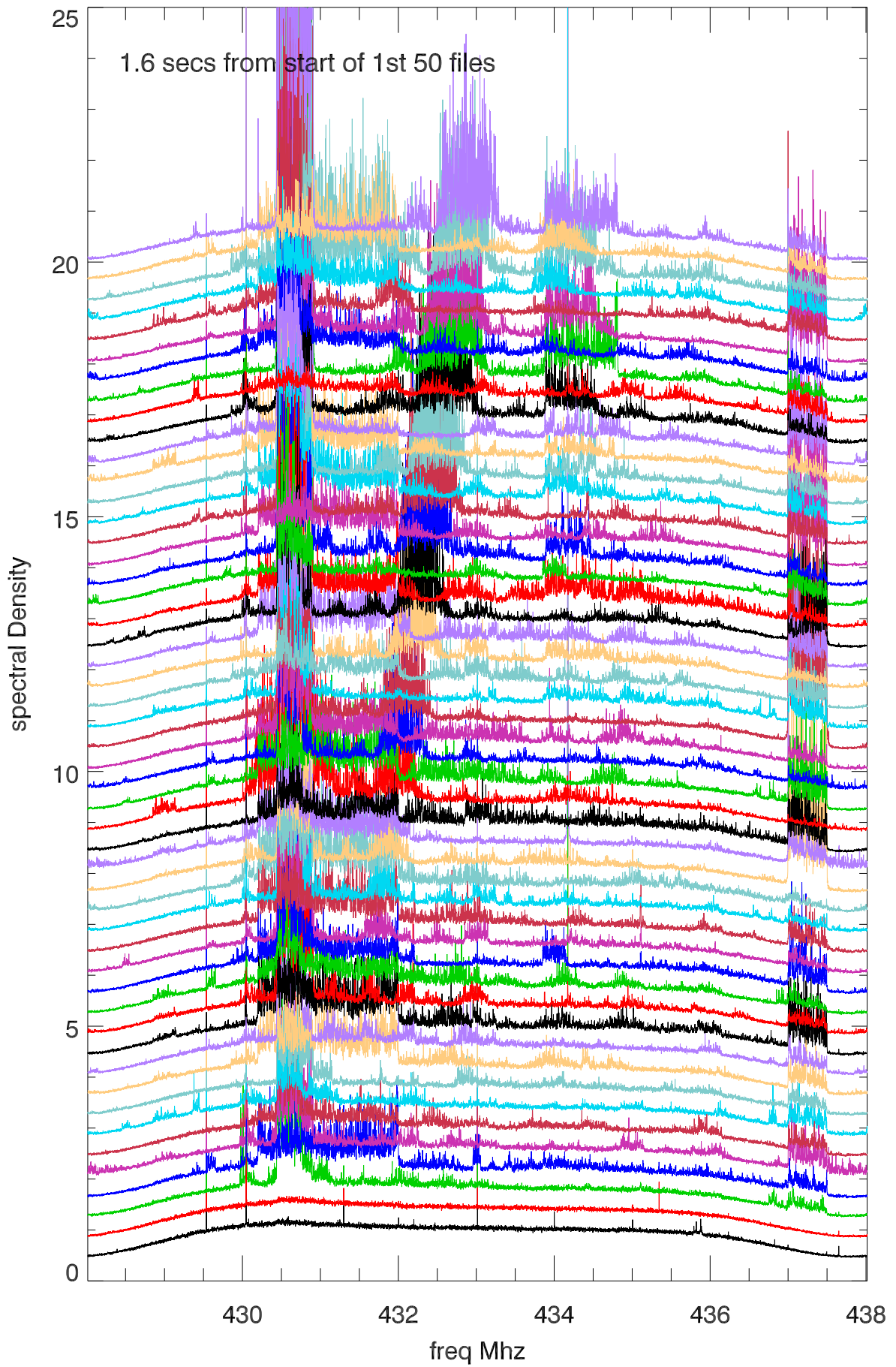
06may14 17:01 to 17:53 (ast) spectral density. polA
