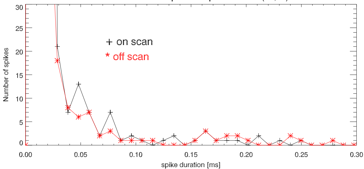
190113 Number of spikes vs spike duration (on,off)
