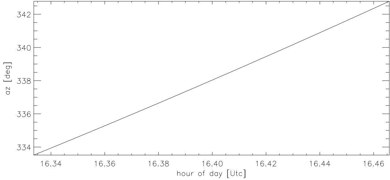
za vs hour of day
