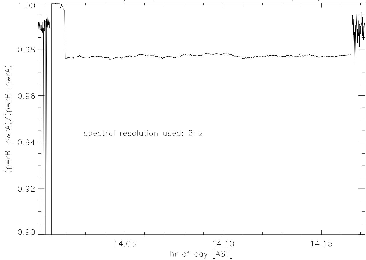
Stokes V/I at peak value of received frequency
