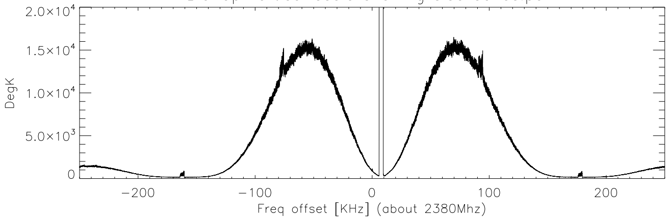
average spectra. PoIB
