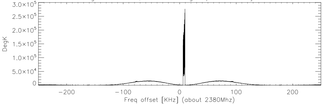
Blowup vertical scale showing side bands.pola
