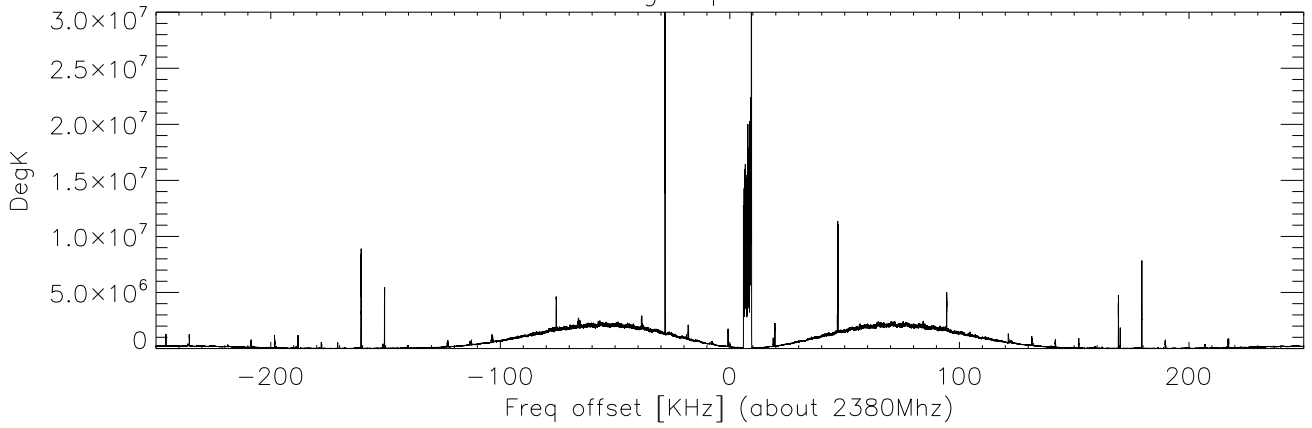
Blowup vertical scale showing side bands polB
