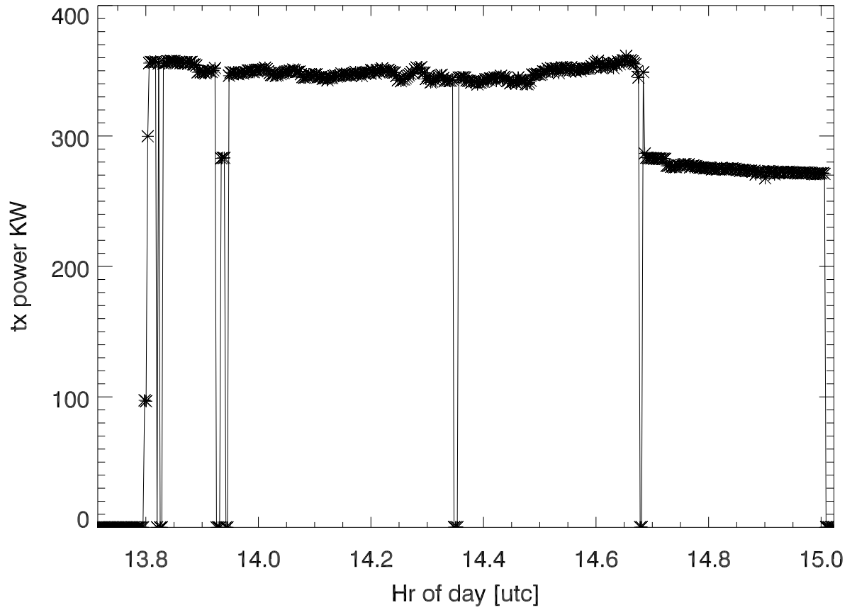
r3399 SbTx transmitted power. 27oct19
