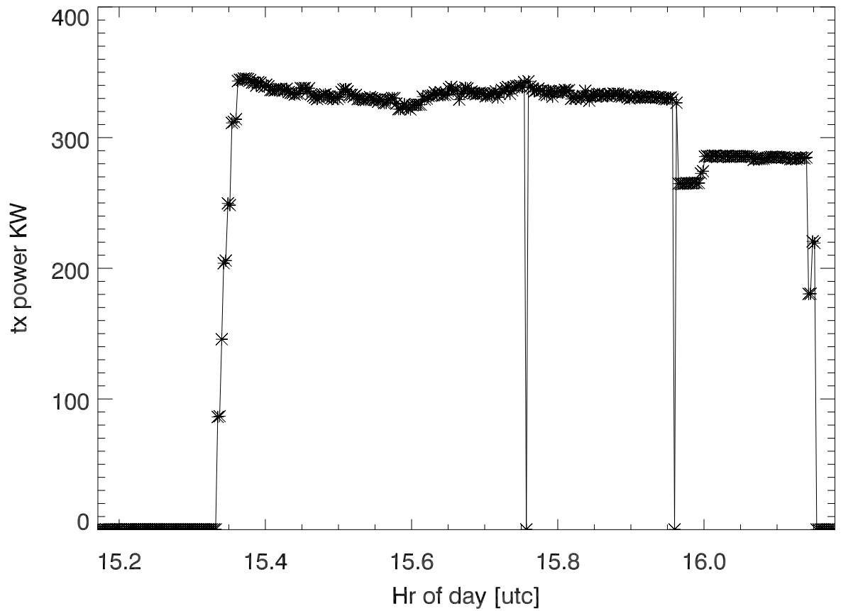
r3399 SbTx transmitted power. 28oct19
