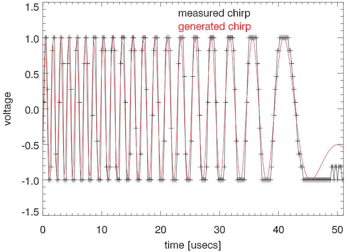
14may12 Ir chirp. measured and generated. Inphase
