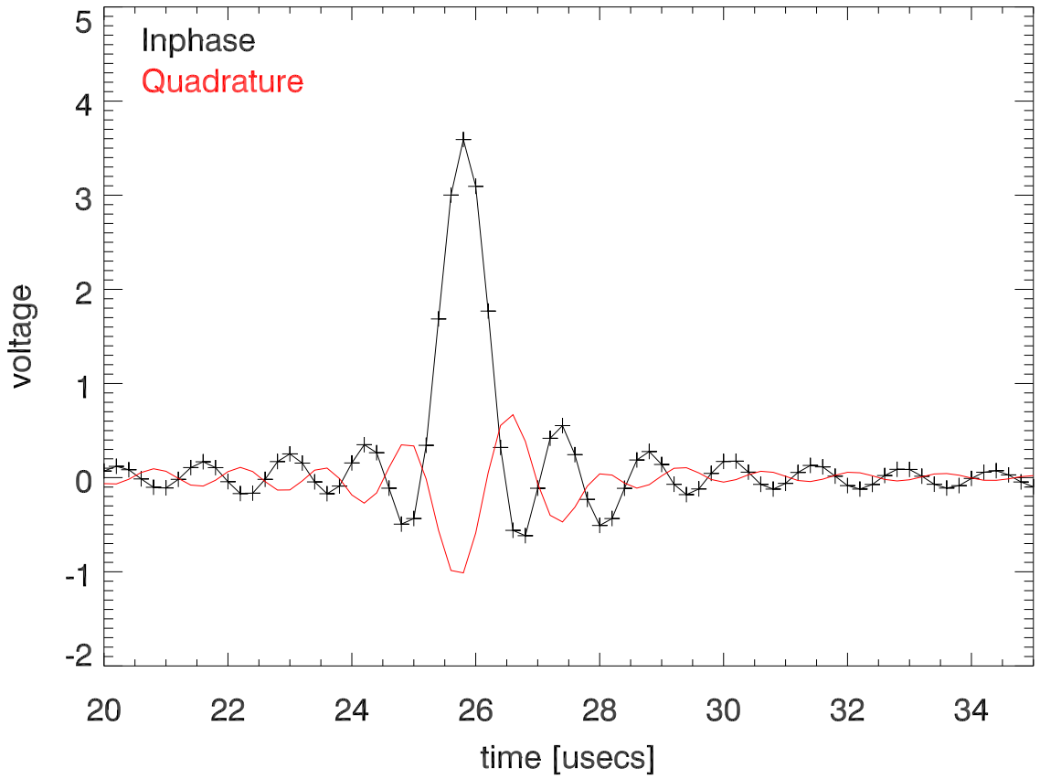
avg .625 secs of voltage data after pulse compression
