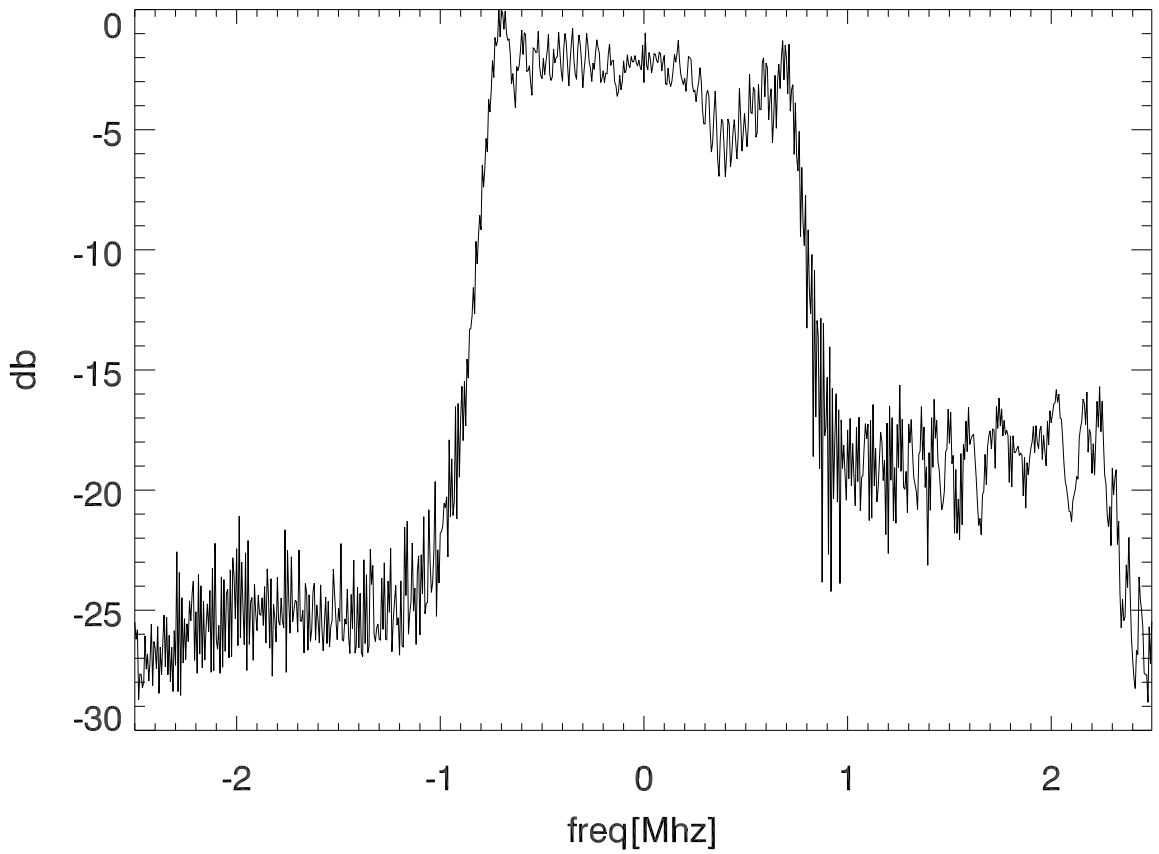
14may12 Iro test. 30 secs avg spectra of chirped xmit signal
