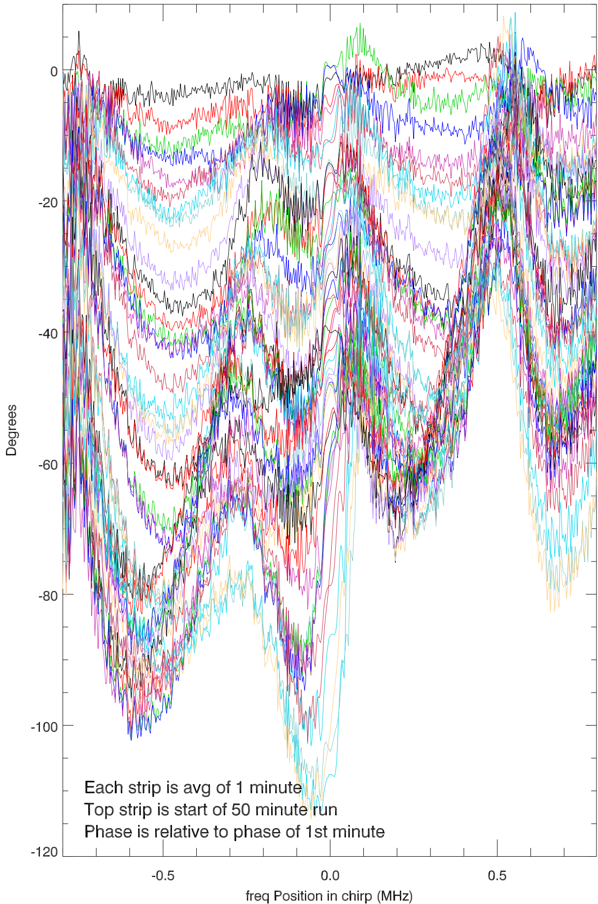
16may Iro. phase change in chirp vs position in chirp for 50 minutes
