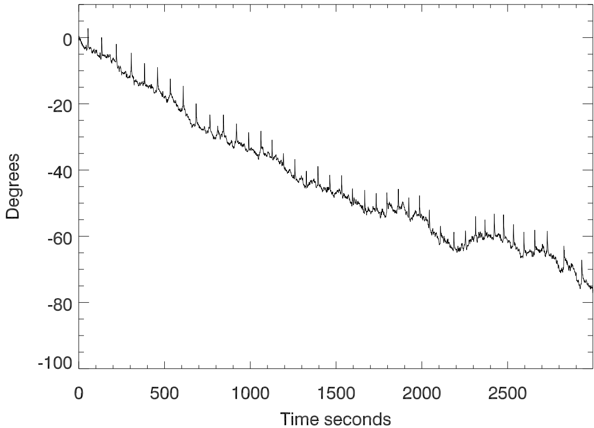
Average phase (averaged over entire chirps) vs time
