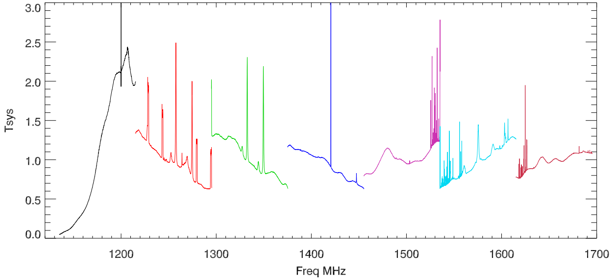
19oct16: p3094 lbw avg spectra (On scans) vs freq for scan:629300050 04:31:58
