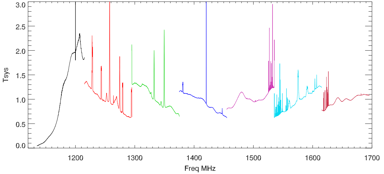
19oct16: p3094 lbw avg spectra (On scans) vs freq for scan:629300034 03:49:57
