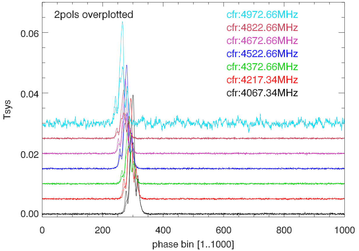
overplot folded freq bands (with offsets for display)
