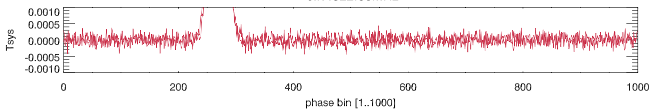
cfr:4972.66MHz
