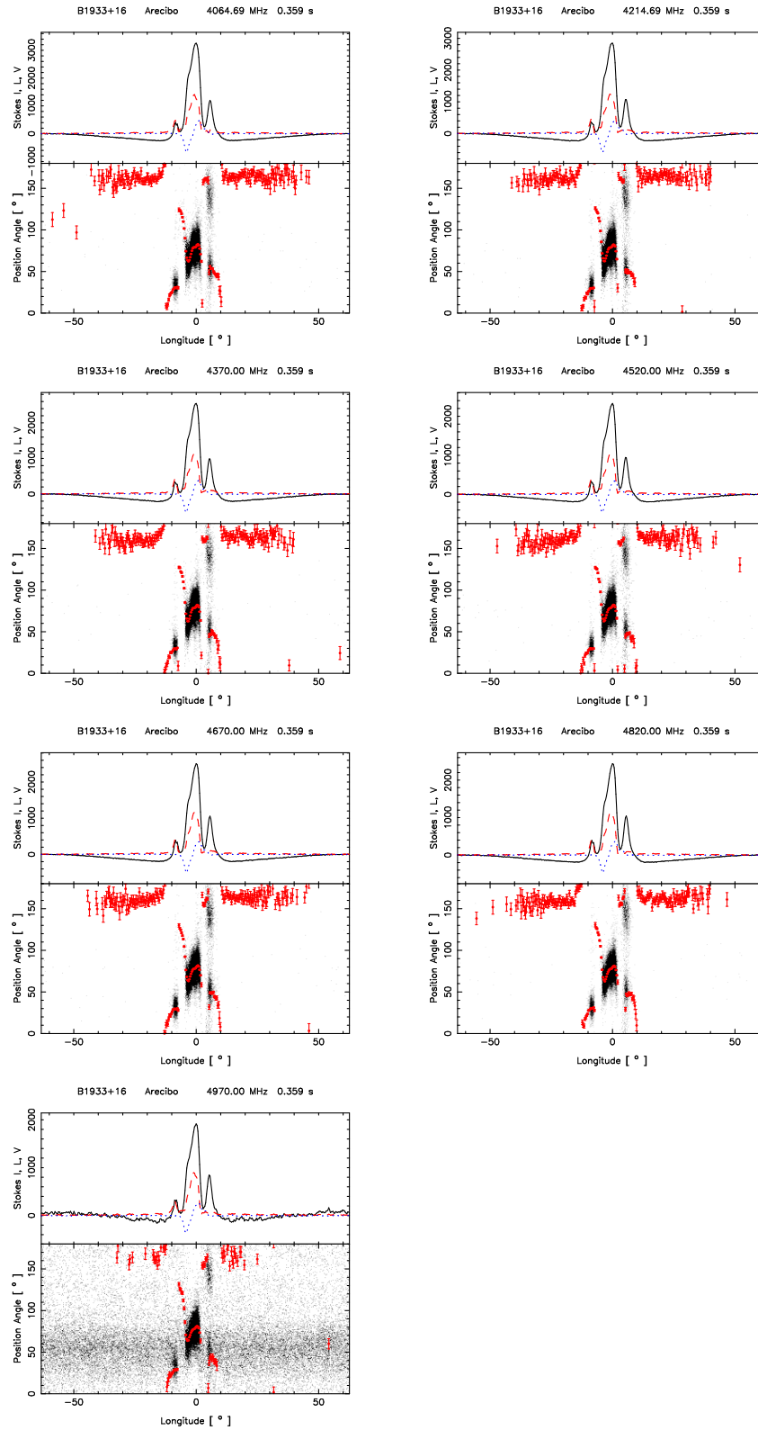
Figure 3: PSR B1933+16 observed on 20th September 2015, 7 mock bands
