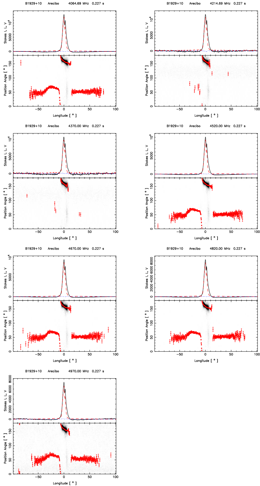
Figure 1: PSR B1929+10 observed on 18th September 2015, 7 mock bands. In each plot, top panel show total intensity in black, linear polarization in red and circular in blue. The bottom panel shows the position angle histogram as dotted plots and the average position angle in red.
