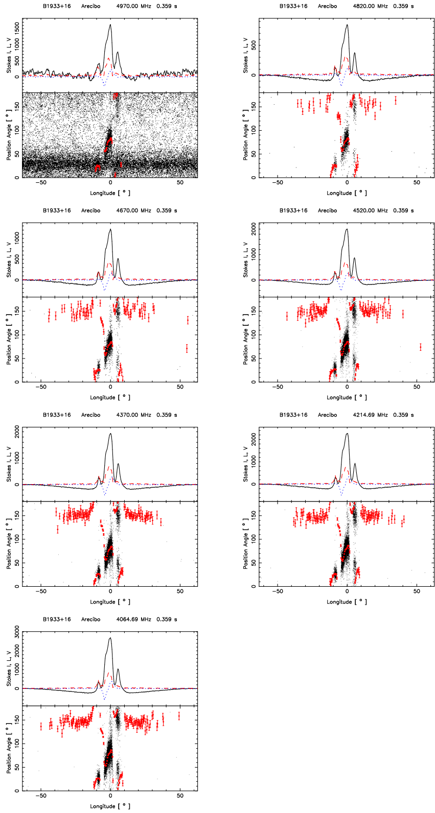
Figure 2: PSR B1933+16 observed on 18th September 2015, 7 mock bands
