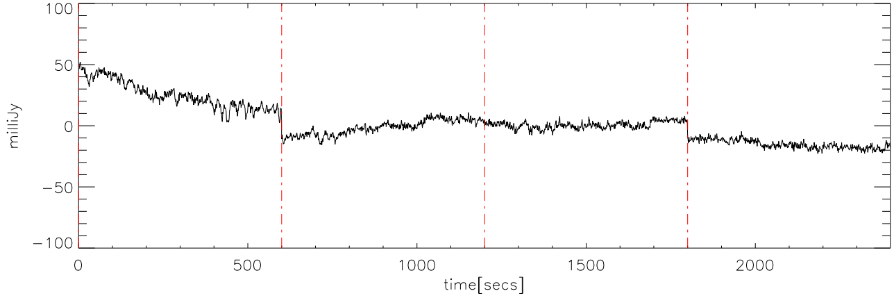
p2111 file:12 29dec08 (AST) StokesQ freq:5000.
