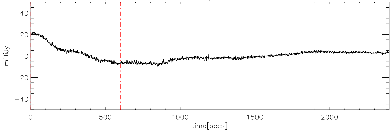
p2111 file:12 29dec08 (AST) StokesU freq:4725.
