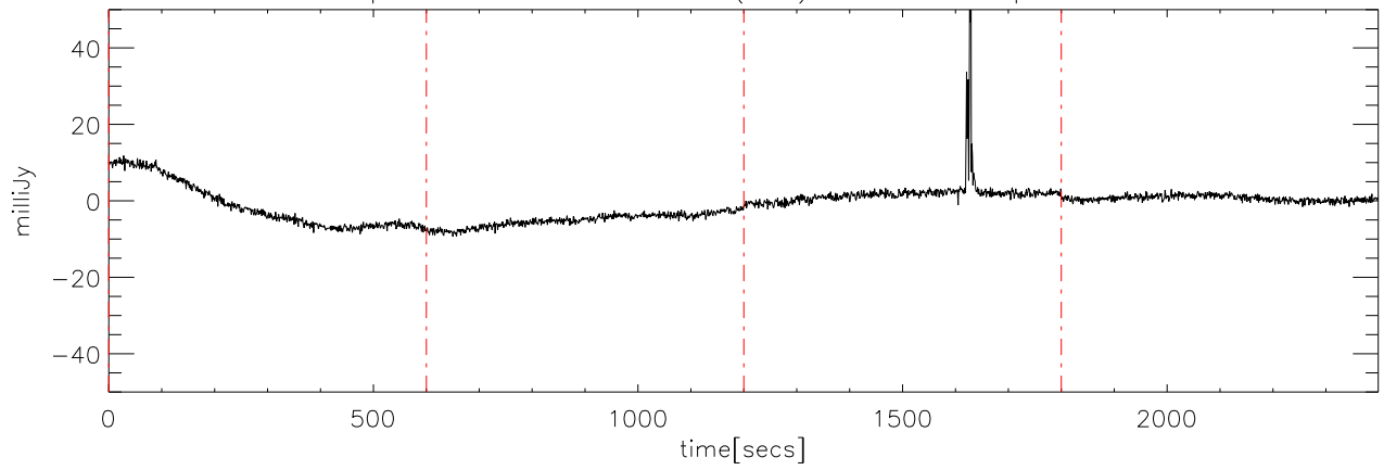
p2111 file:12 29dec08 (AST) StokesU freq:4600.
