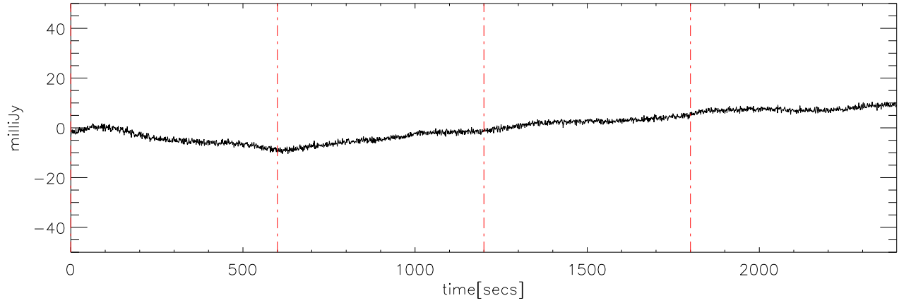
p2111 file:12 29dec08 (AST) StokesU freq:5000.
