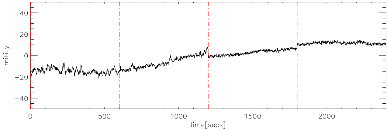
p2111 file:12 29dec08 (AST) StokesU freq:5250.
