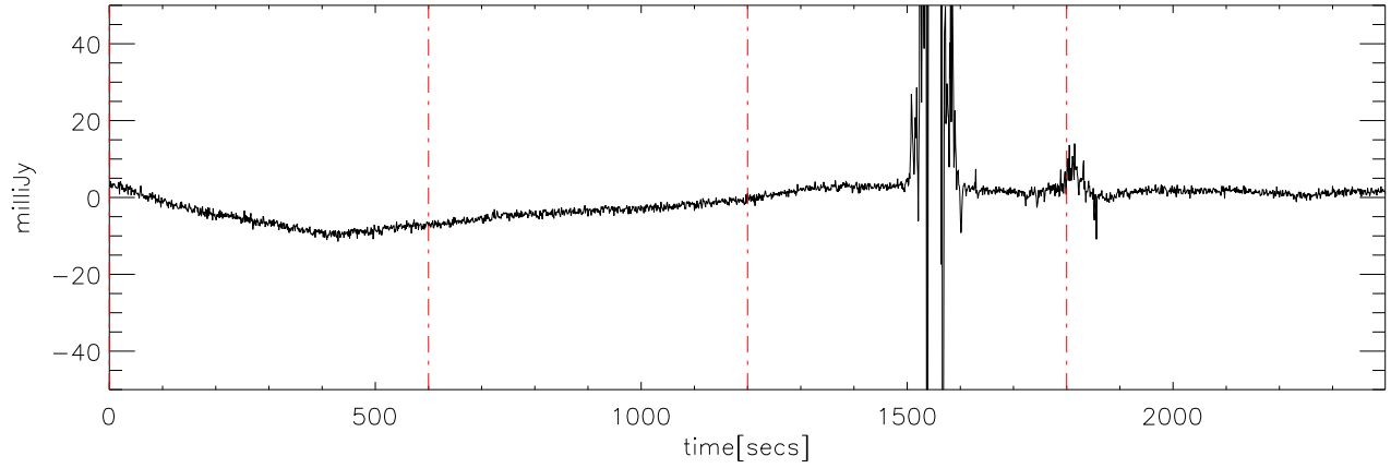
p2111 file:12 29dec08 (AST) StokesU freq:4475.
