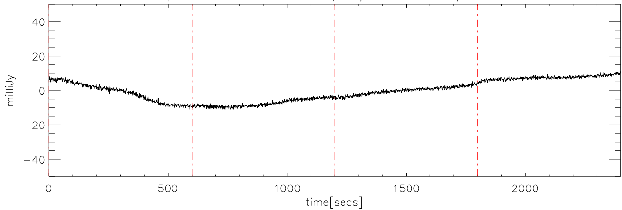
p2111 file:12 29dec08 (AST) StokesU freq:5125.
