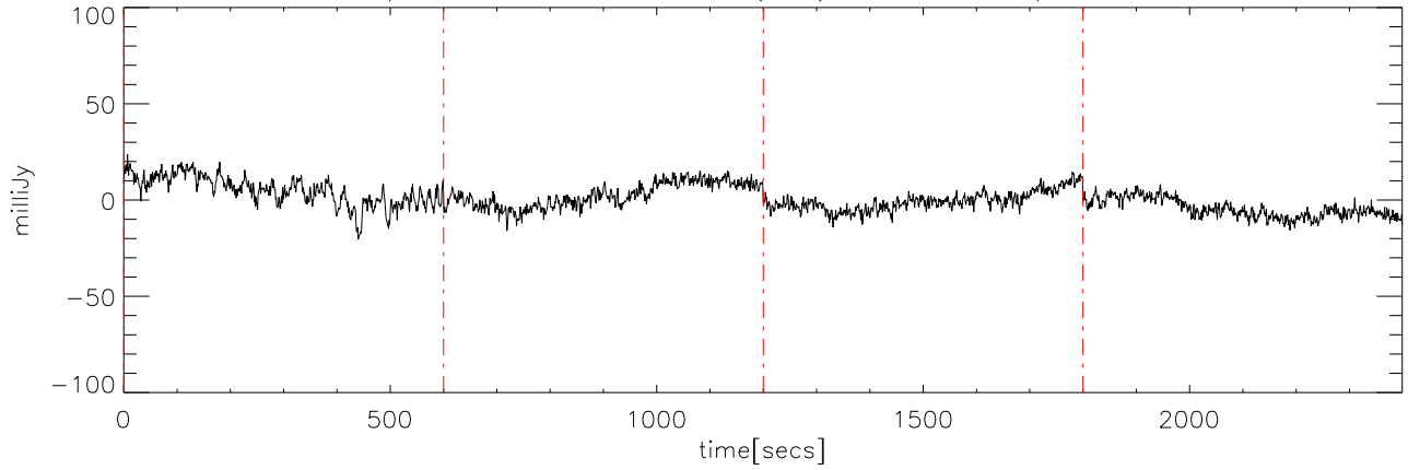
p2111 file:12 29dec08 (AST) StokesQ freq:5250.
