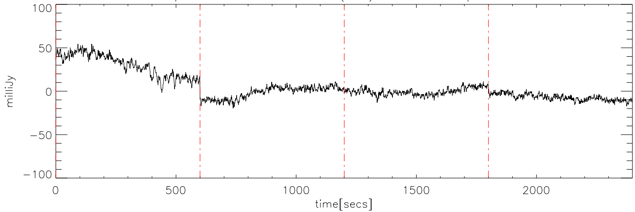
p2111 file:12 29dec08 (AST) StokesQ freq:5125.
