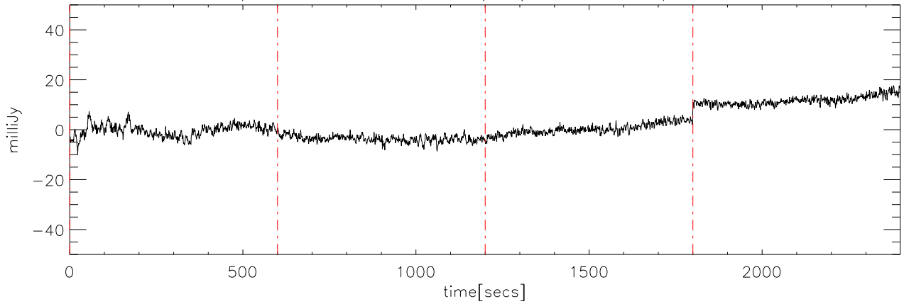
p2111 file:08 30dec08 (AST) StokesU freq:5250.
