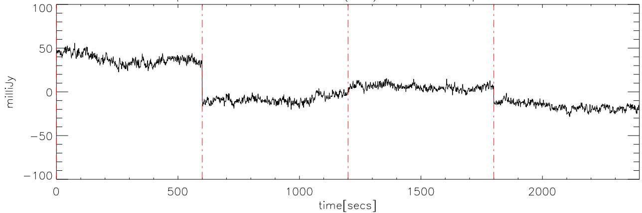
p2111 file:08 30dec08 (AST) StokesQ freq:5250.
