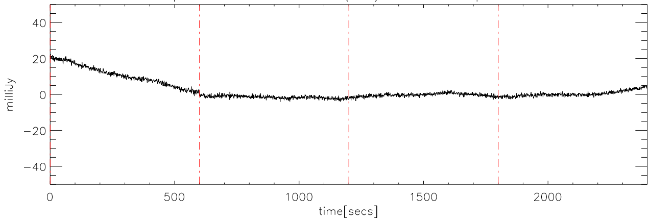
p2111 file:08 30dec08 (AST) StokesU freq:5125.
