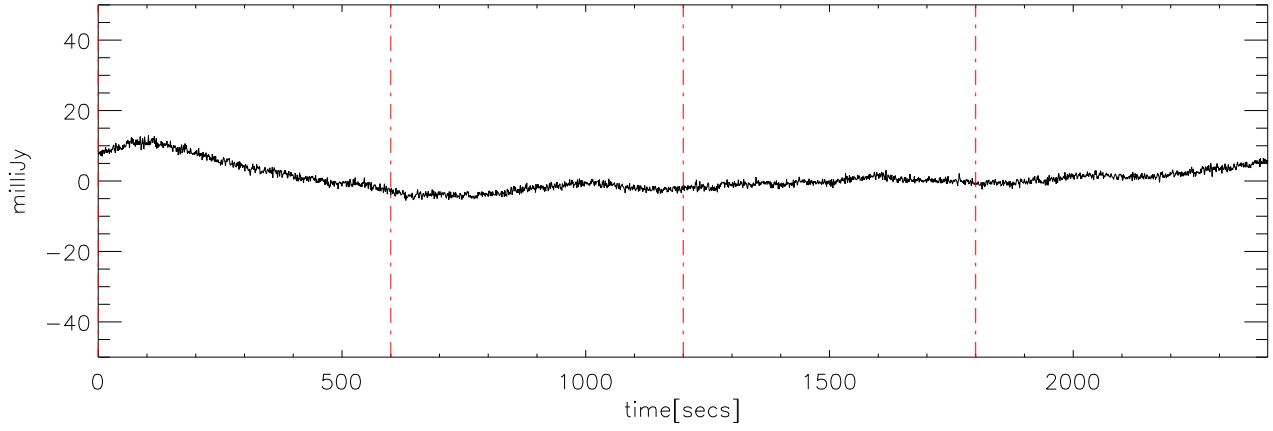
p2111 file:08 30dec08 (AST) StokesU freq:5000.
