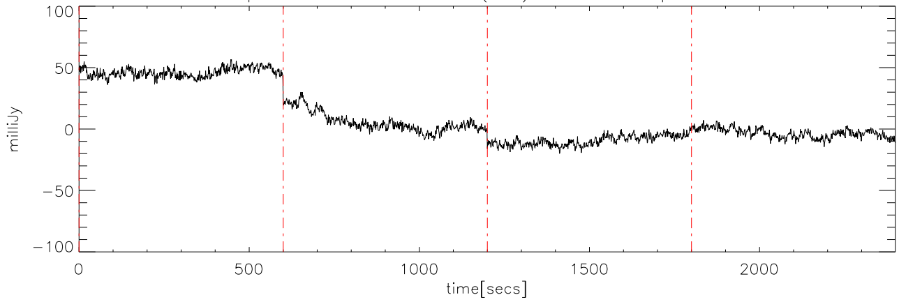
p2111 file:08 30dec08 (AST) StokesQ freq:5125.
