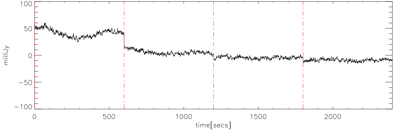
p2111 file:08 30dec08 (AST) StokesQ freq:5000.
