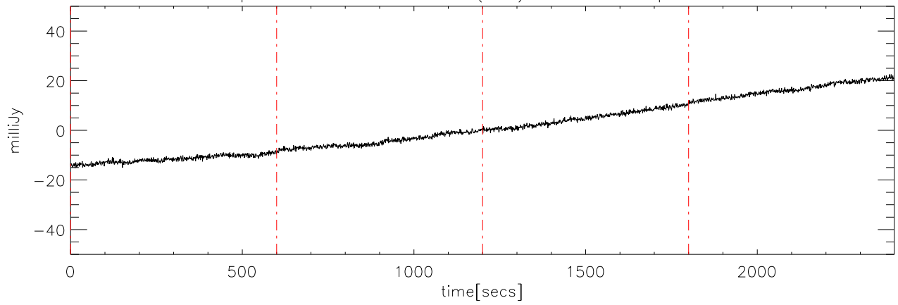
p2111 file:08 29dec08 (AST) StokesU freq:4600.
