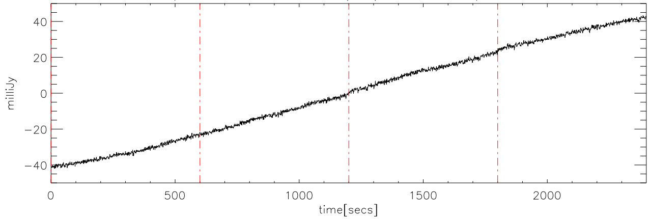
p2111 file:08 29dec08 (AST) StokesU freq:5250.
