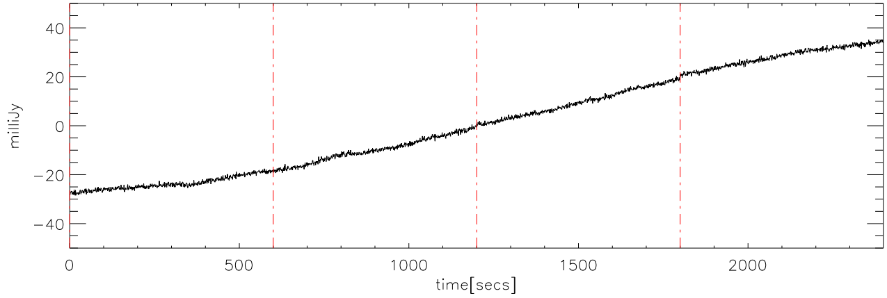
p2111 file:08 29dec08 (AST) StokesU freq:5000.
