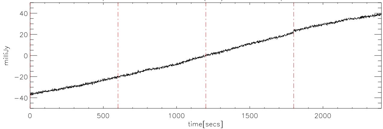
p2111 file:08 29dec08 (AST) StokesU freq:5125.
