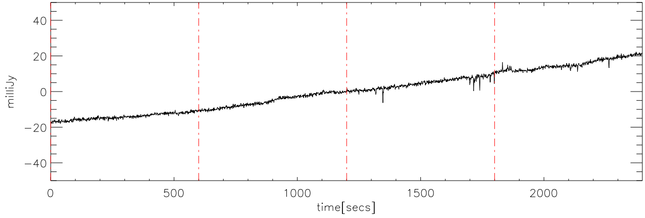
p2111 file:08 29dec08 (AST) StokesU freq:4475.
