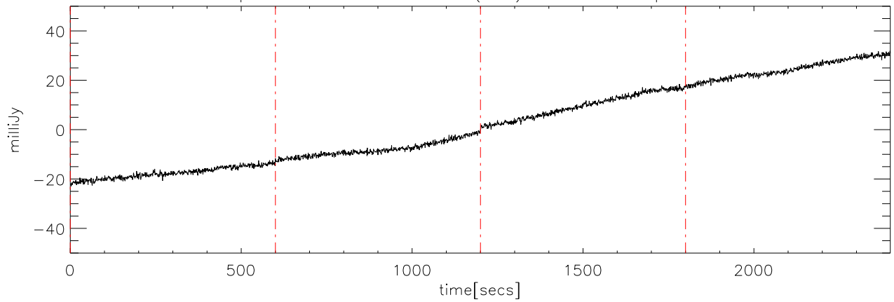
p2111 file:08 29dec08 (AST) StokesU freq:4725.
