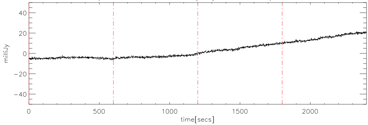
p2111 file:00 30dec08 (AST) StokesU freq:4600.
