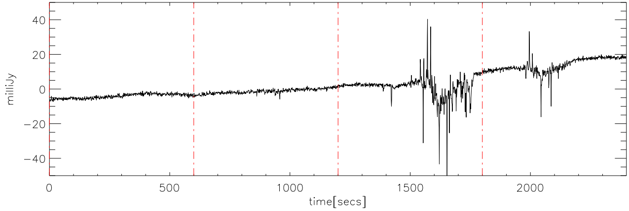
p2111 file:00 30dec08 (AST) StokesU freq:4475.
