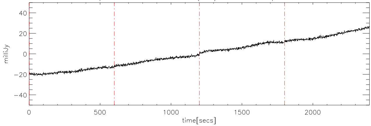
p2111 file:00 30dec08 (AST) StokesU freq:5125.
