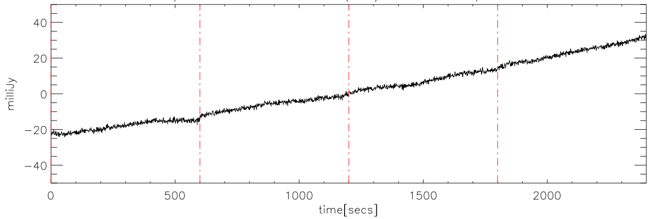
p2111 file:00 30dec08 (AST) StokesU freq:5250.
