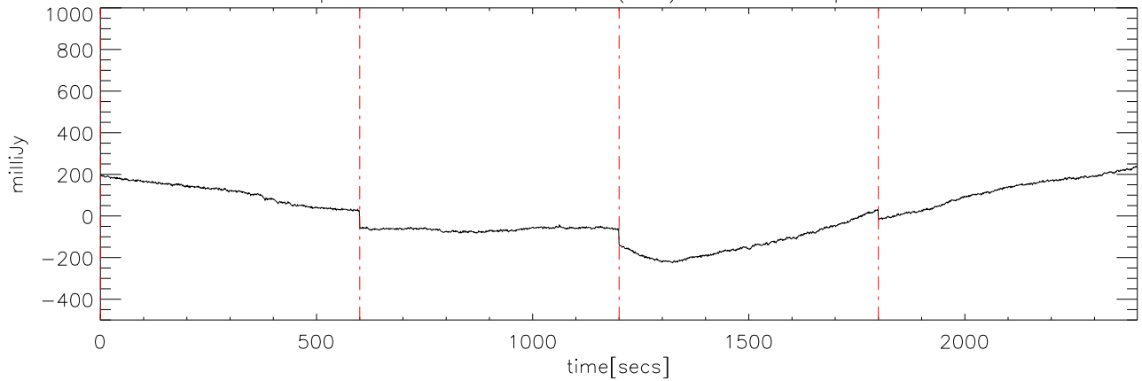
p2111 file:00 30dec08 (AST) StokesI freq:5125.
