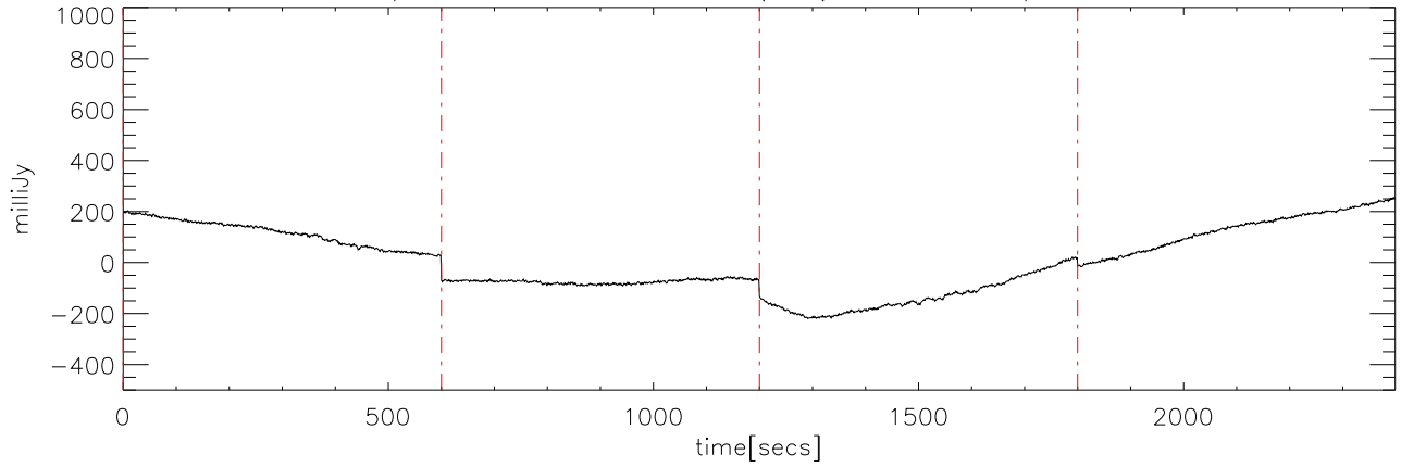
p2111 file:00 30dec08 (AST) StokesI freq:5250.
