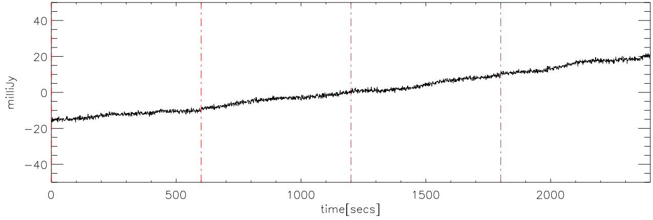
p2111 file:00 30dec08 (AST) StokesU freq:5000.
