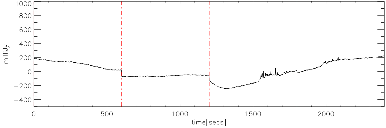
p2111 file:00 30dec08 (AST) StokesI freq:4475.
