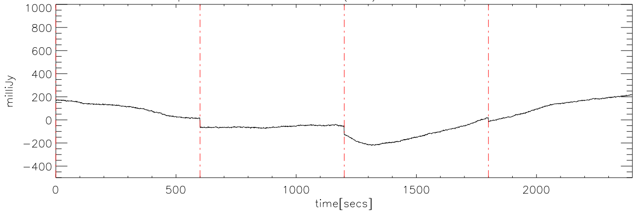
p2111 file:00 30dec08 (AST) StokesI freq:4600.
