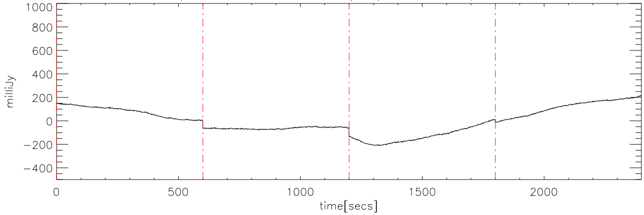
p2111 file:00 30dec08 (AST) StokesI freq:4725.
