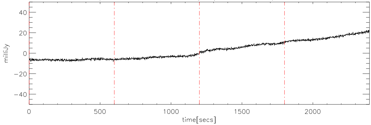
p2111 file:00 30dec08 (AST) StokesU freq:4725.
