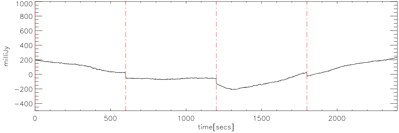
p2111 file:00 30dec08 (AST) StokesI freq:5000.
