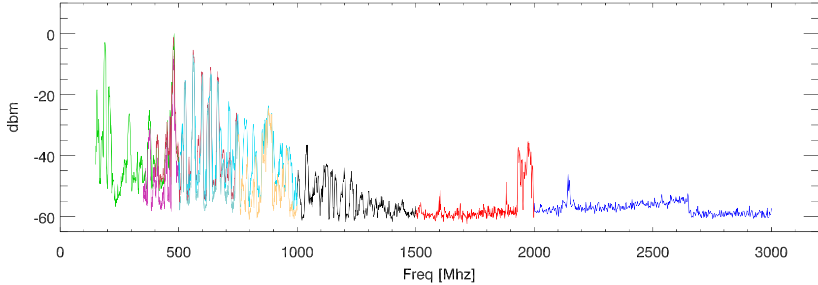
15may13 spectrum Analyzer @ lincoln Lab Ina + 10db pad
