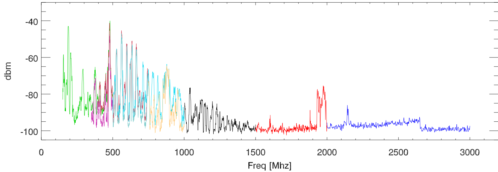
spectral density at output of lincoln Lab antenna
