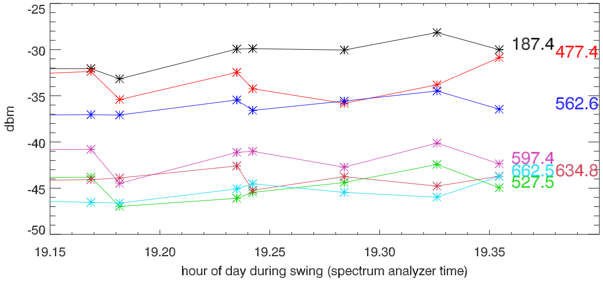
Birdie peak variation during azswing.SpecAna value
