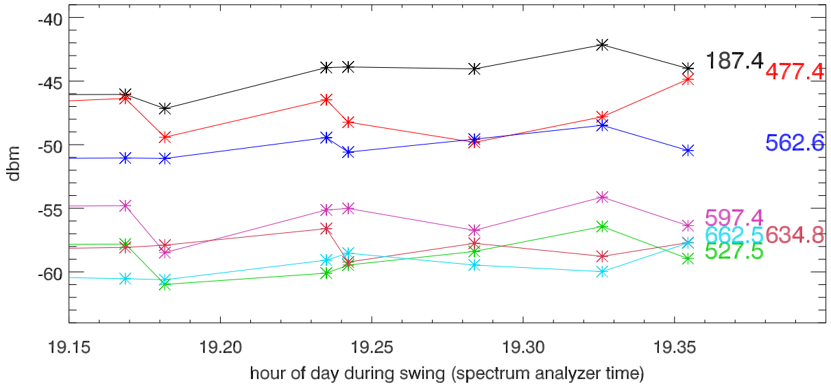
Birdie peak variation at output of Antenna
