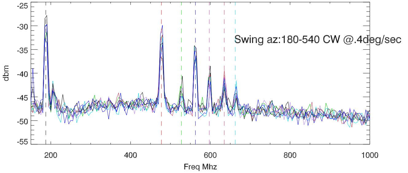
20may13 spectral density during lincolLab az swing. specAna value
