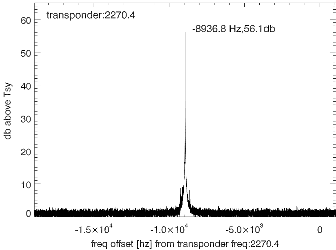
isee3 140627:195733 (UTC) spectra after doppler correction. PolA
