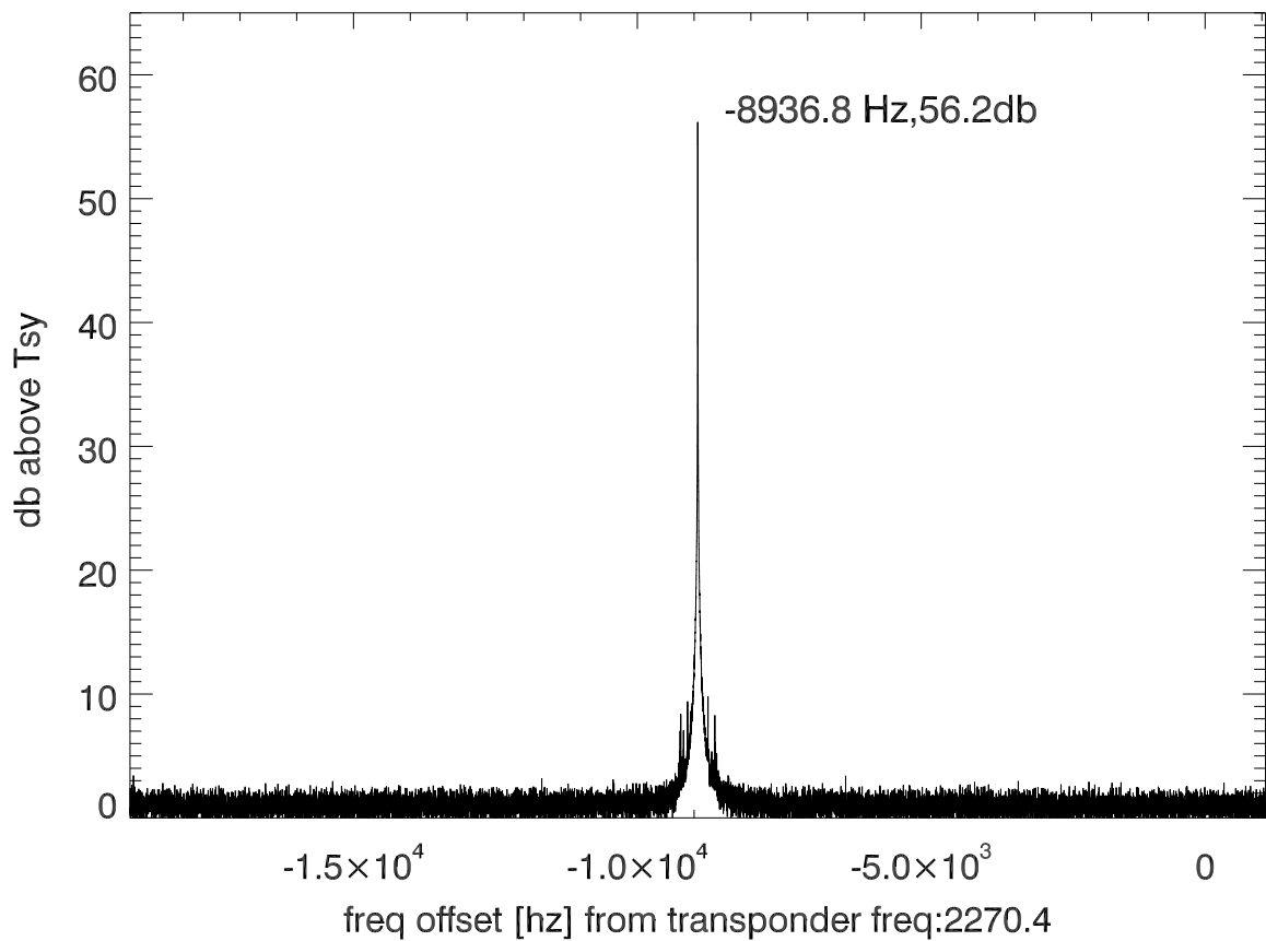
isee3 140627:195733 (UTC) spectra after doppler correction. PolB
