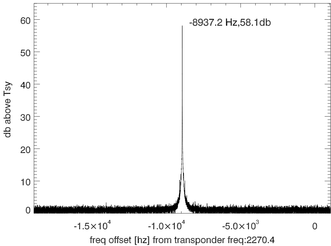
isee3 140627:195053 (UTC) spectra after doppler correction. PolB
