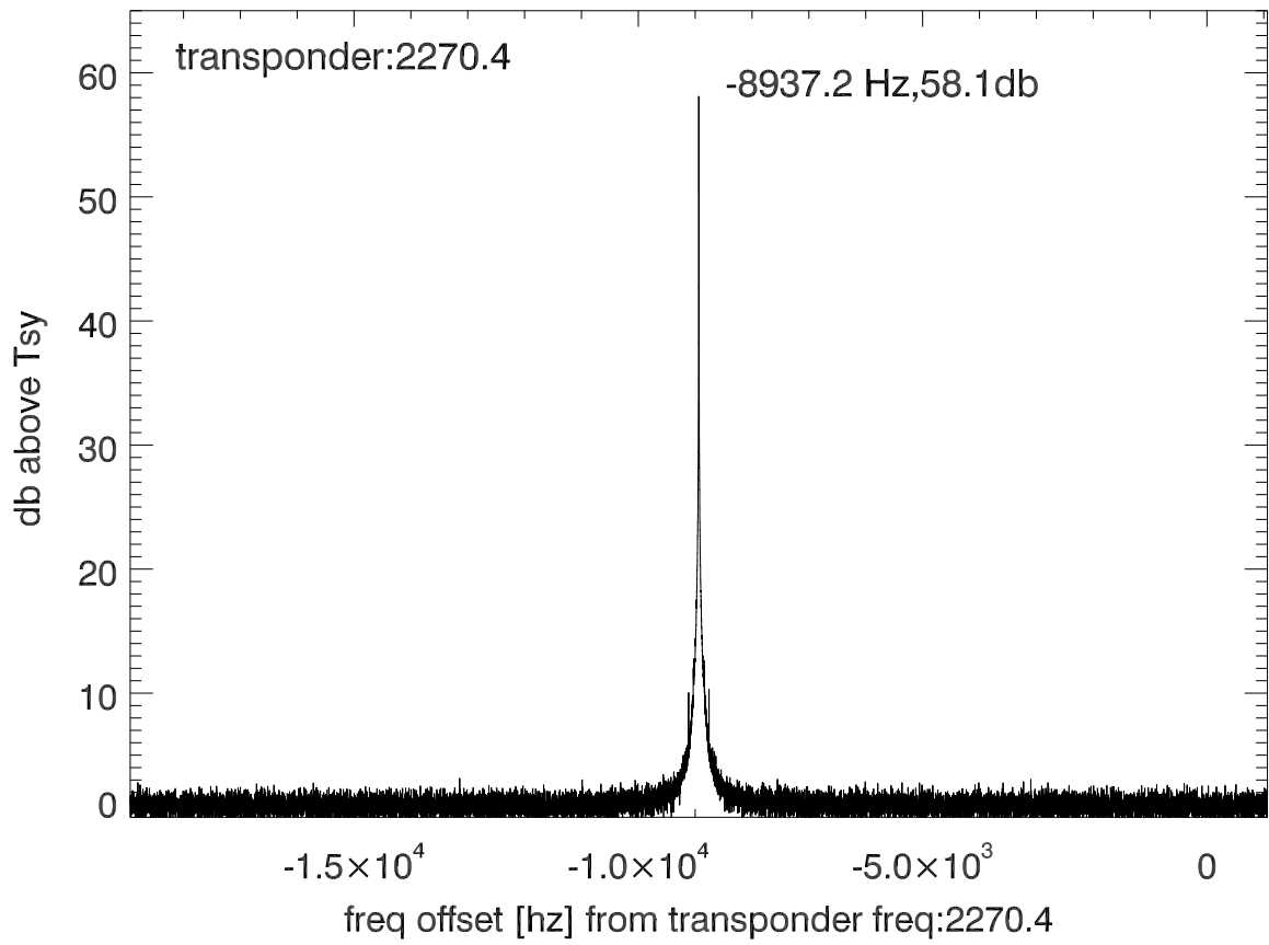
isee3 140627:195053 (UTC) spectra after doppler correction. PolA
