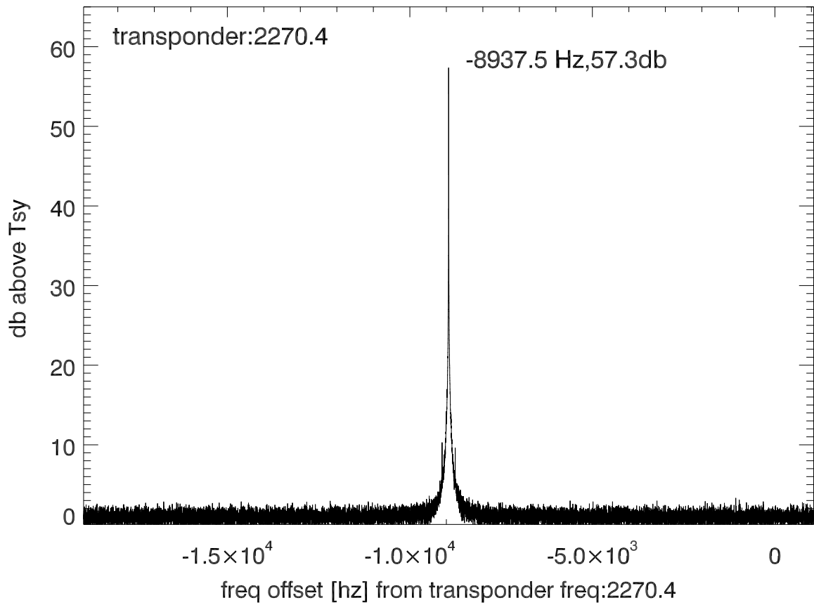
isee3 140627:194829 (UTC) spectra after doppler correction. PolA
