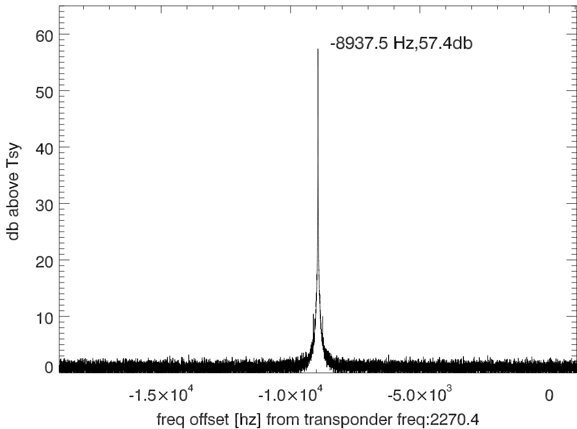
isee3 140627:194829 (UTC) spectra after doppler correction. PolB
