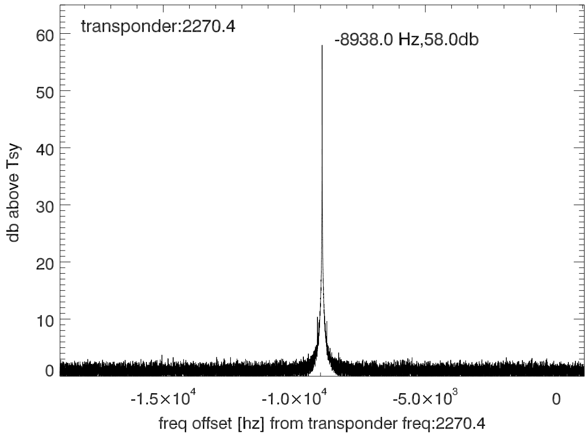
isee3 140627:194216 (UTC) spectra after doppler correction. PolA
