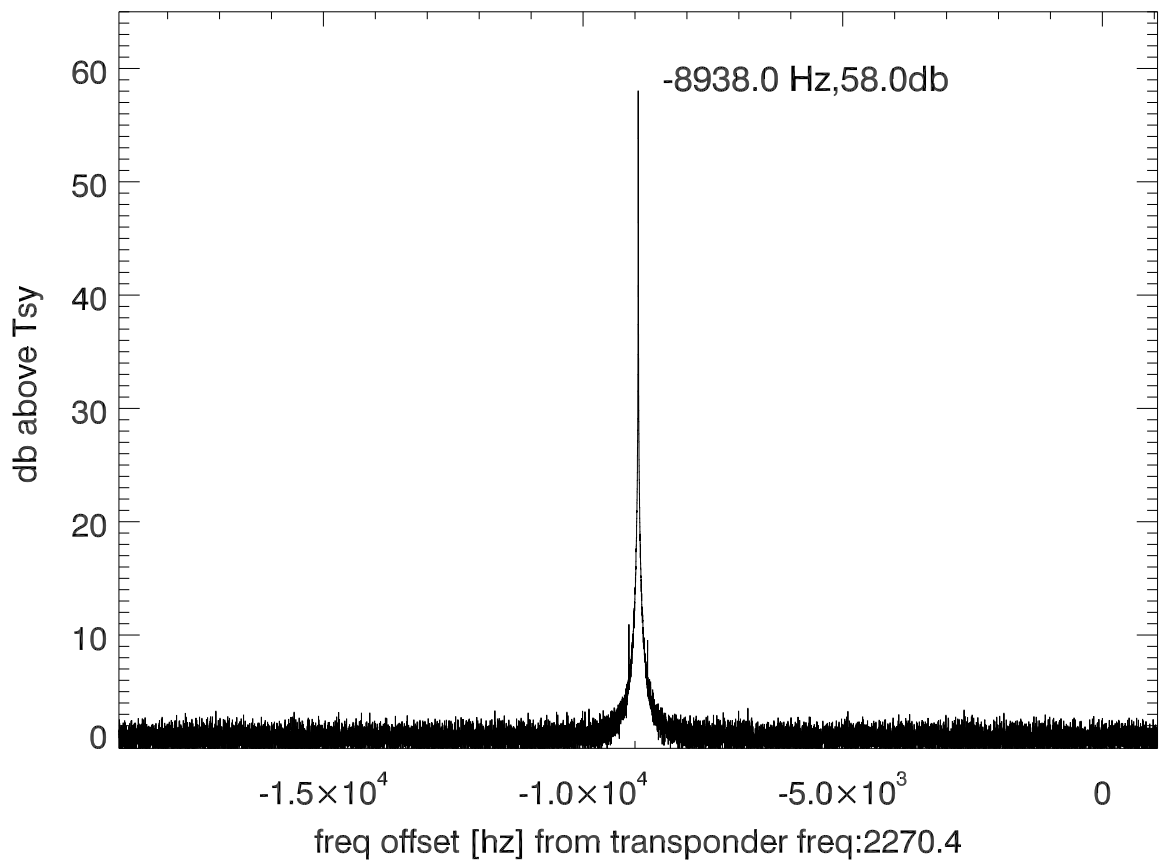
isee3 140627:194216 (UTC) spectra after doppler correction. PolB
