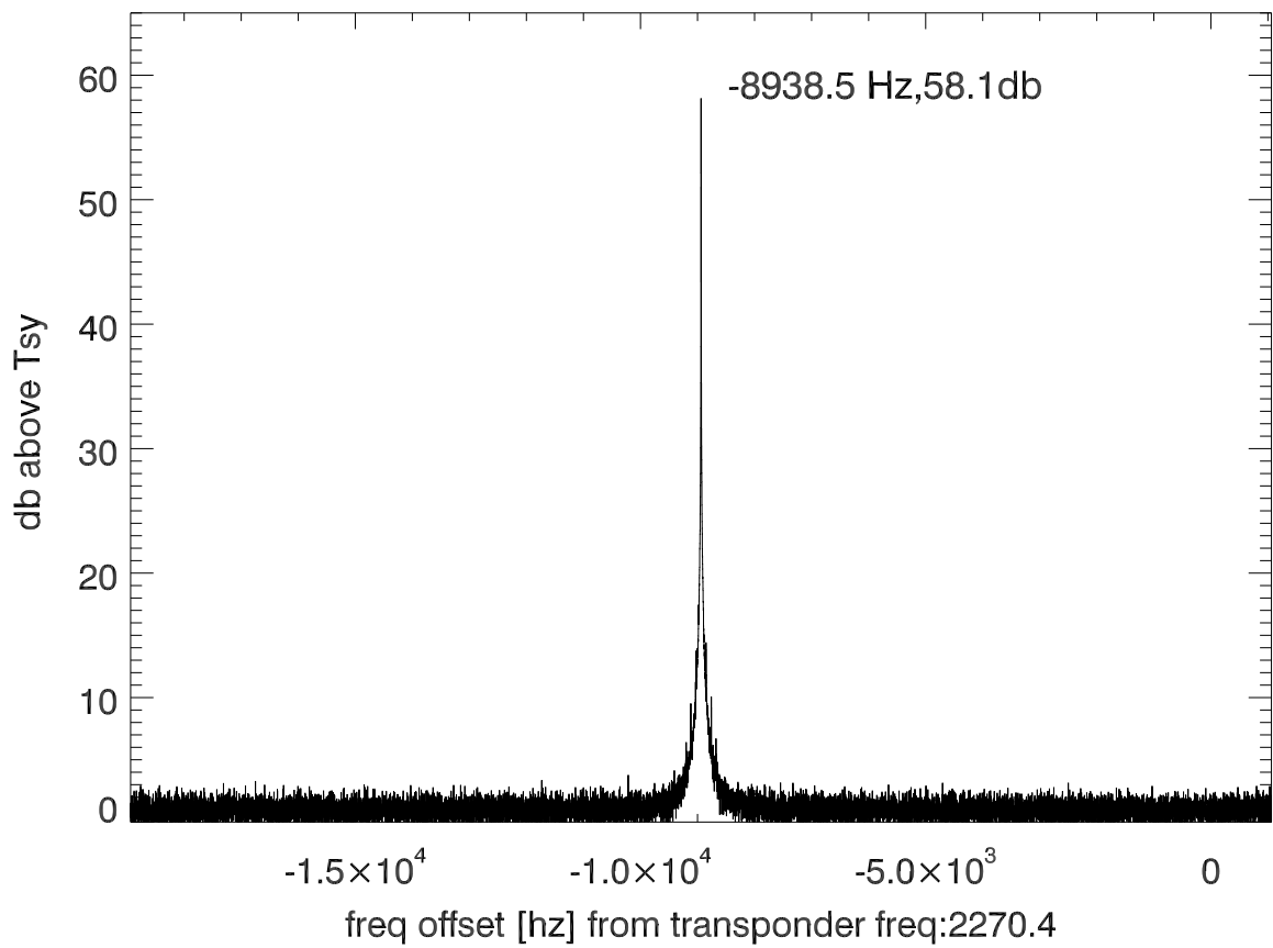
isee3 140627:193605 (UTC) spectra after doppler correction. PolB
