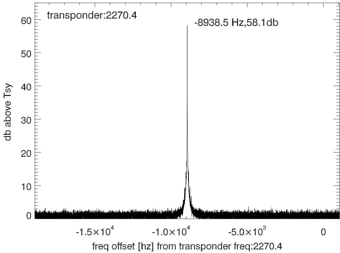
isee3 140627:193605 (UTC) spectra after doppler correction. PolA
