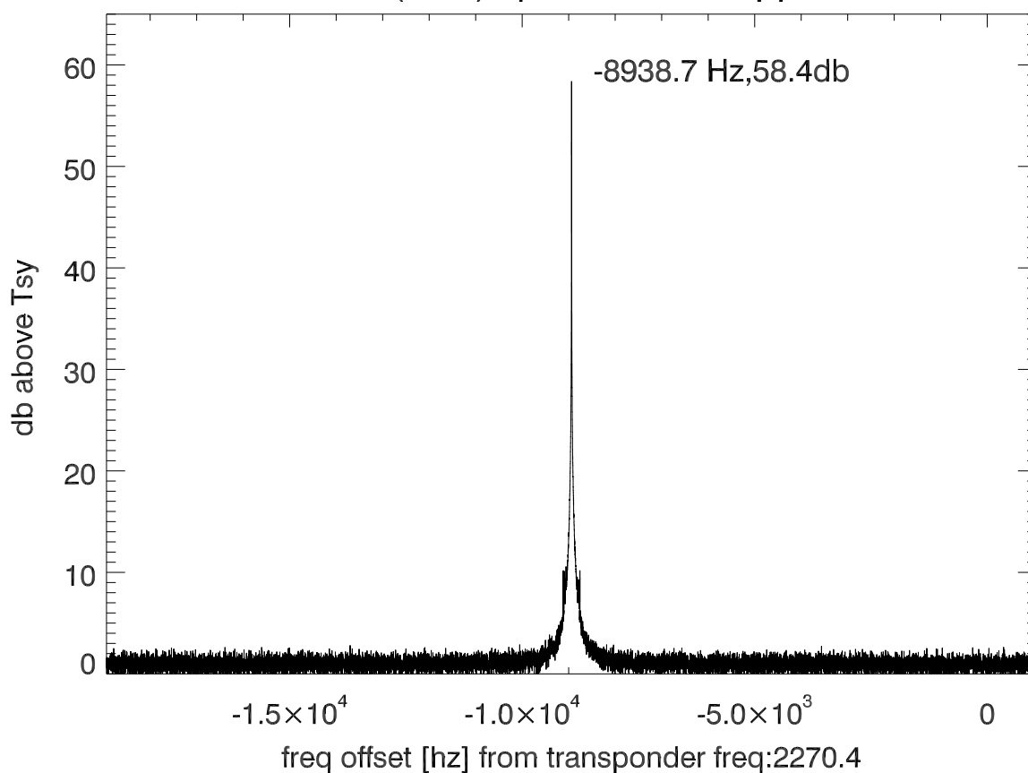
isee3 140627:193333 (UTC) spectra after doppler correction. PolB
