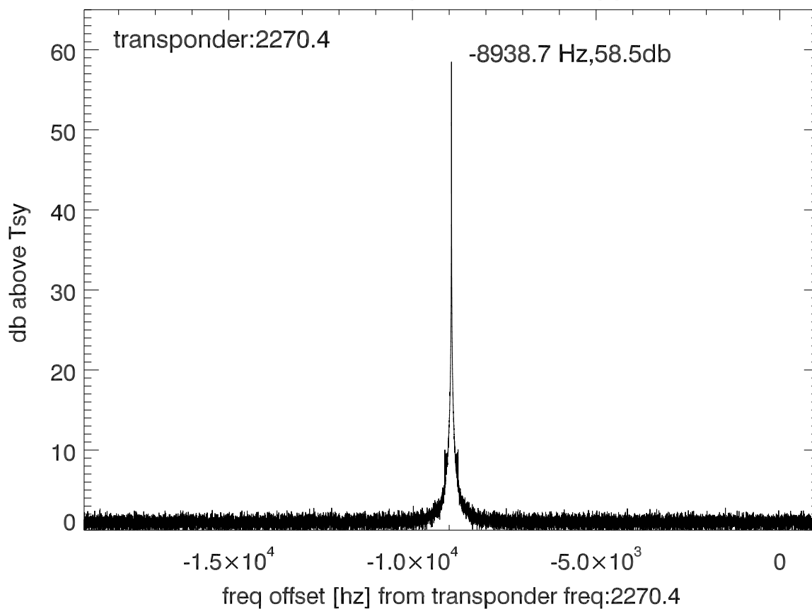
isee3 140627:193333 (UTC) spectra after doppler correction. PolA
