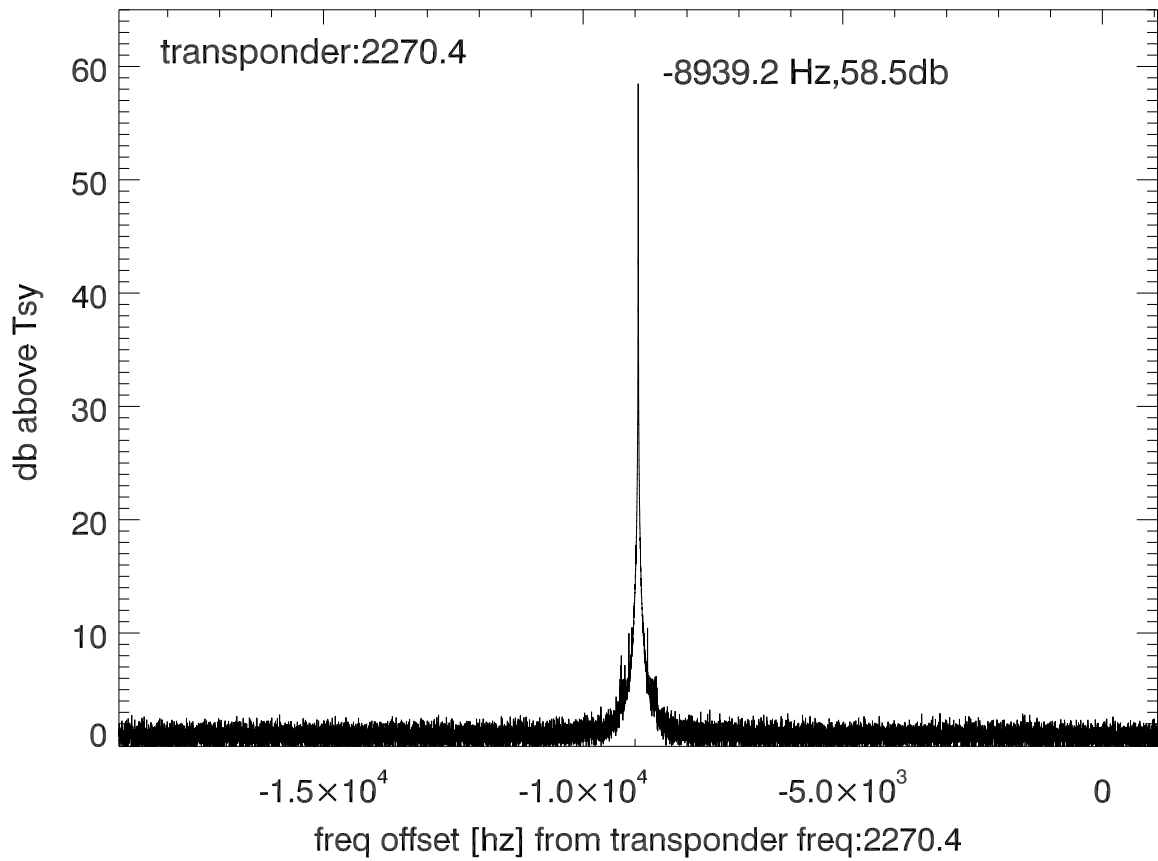
isee3 140627:192629 (UTC) spectra after doppler correction. PolA
