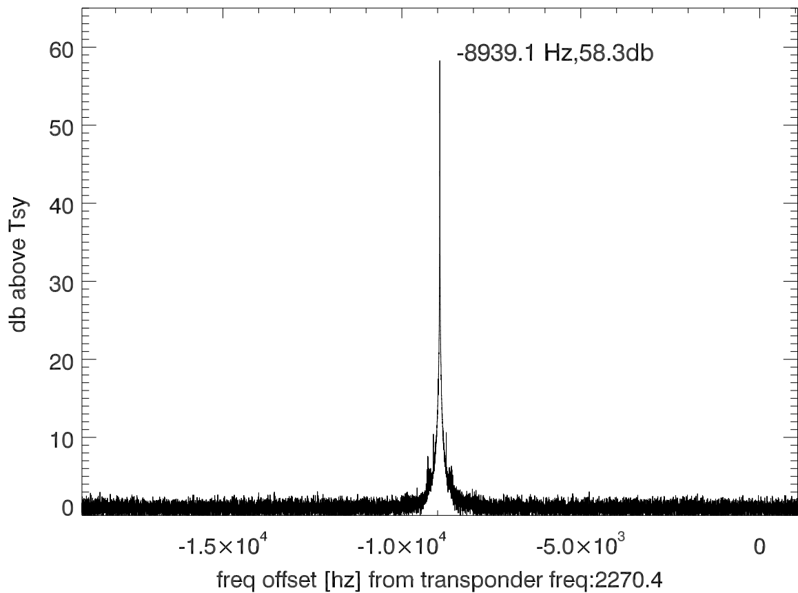
isee3 140627:192629 (UTC) spectra after doppler correction. PolB
