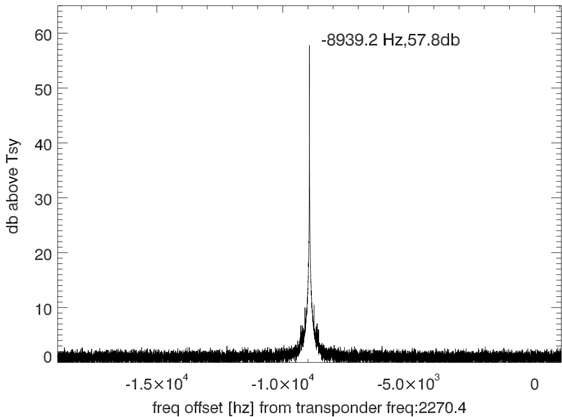
isee3 140627:192349 (UTC) spectra after doppler correction. PolB
