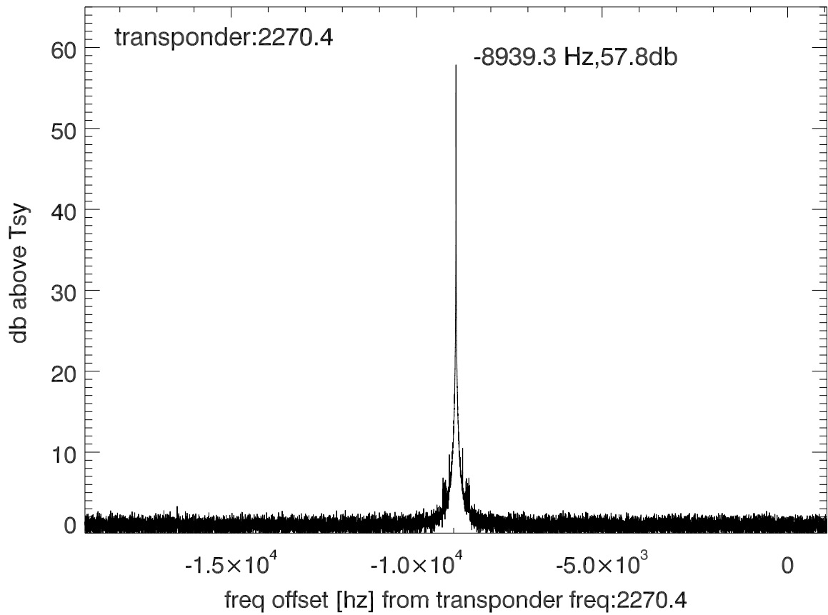
isee3 140627:192349 (UTC) spectra after doppler correction. PolA
