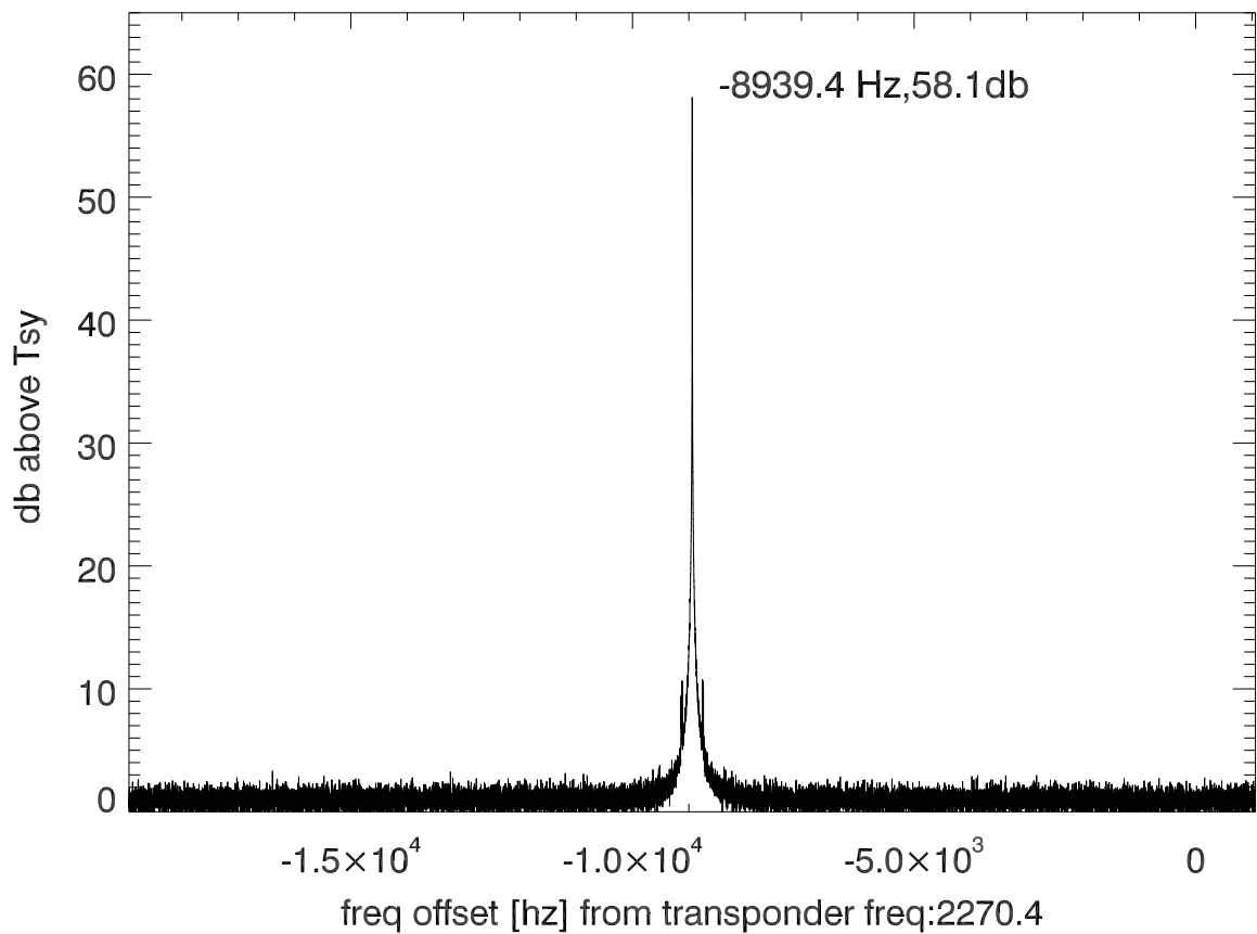
isee3 140627:191525 (UTC) spectra after doppler correction. PolB
