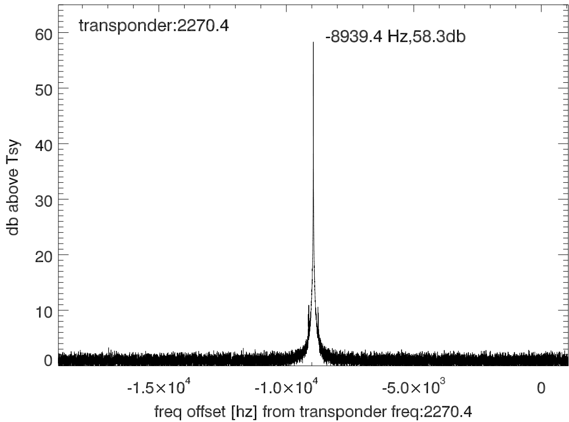
isee3 140627:191525 (UTC) spectra after doppler correction. PolA
