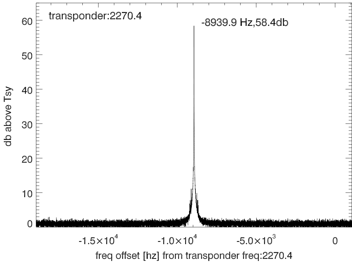
isee3 140627:191045 (UTC) spectra after doppler correction. PolA
