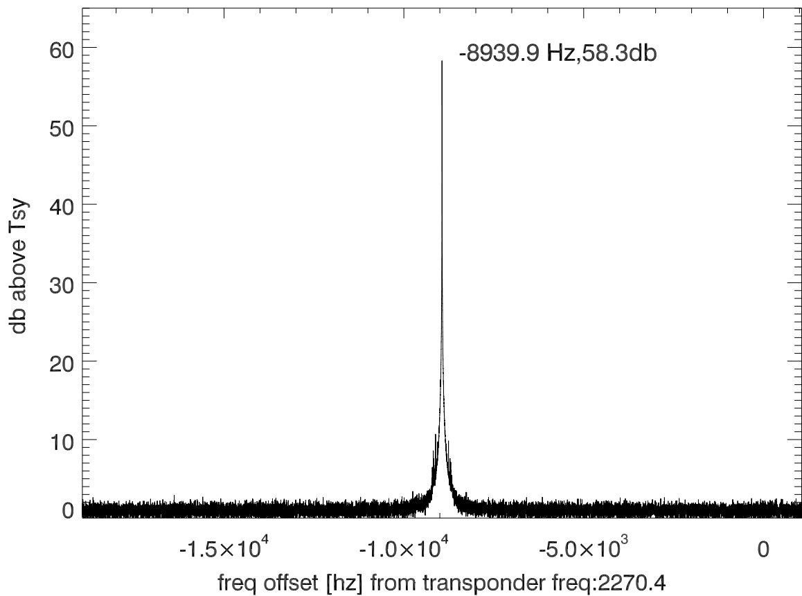
isee3 140627:191045 (UTC) spectra after doppler correction. PolB
