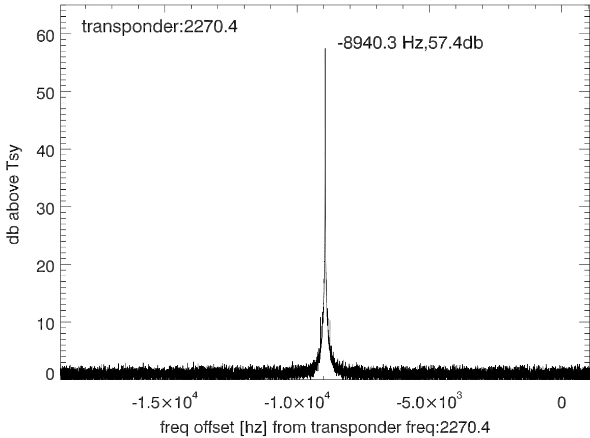
isee3 140627:185329 (UTC) spectra after doppler correction. PolA
