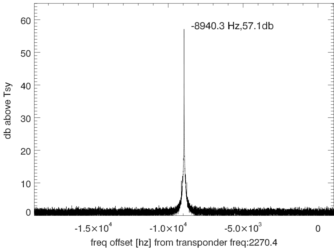
isee3 140627:185329 (UTC) spectra after doppler correction. PolB
