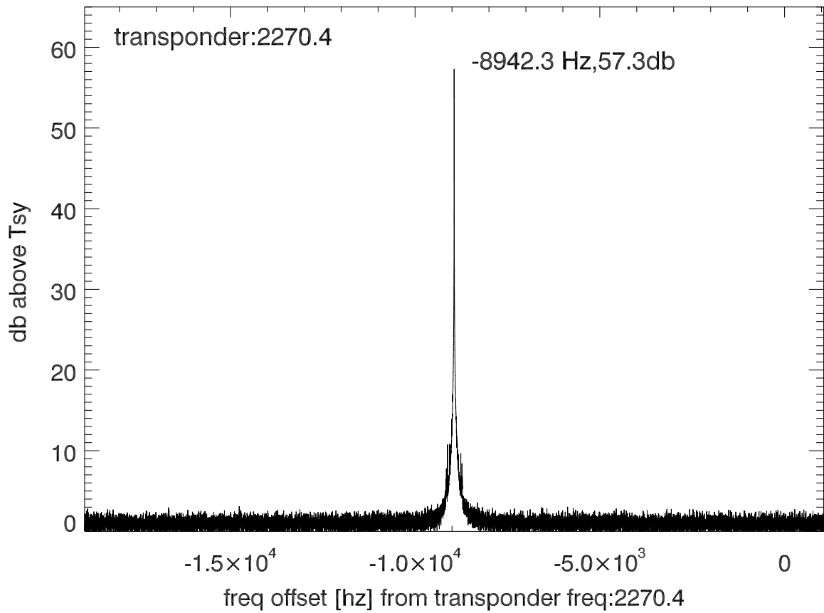
isee3 140627:182715 (UTC) spectra after doppler correction. PolA
