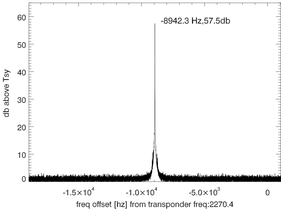
isee3 140627:182715 (UTC) spectra after doppler correction. PolB
