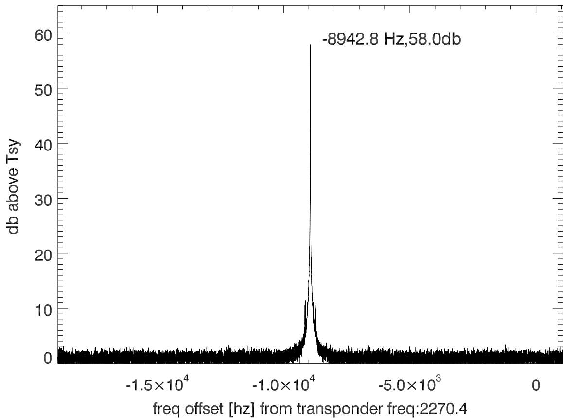
isee3 140627:181630 (UTC) spectra after doppler correction. PolB
