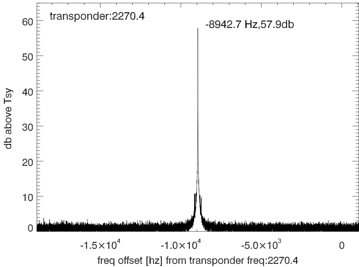
isee3 140627:181630 (UTC) spectra after doppler correction. PolA
