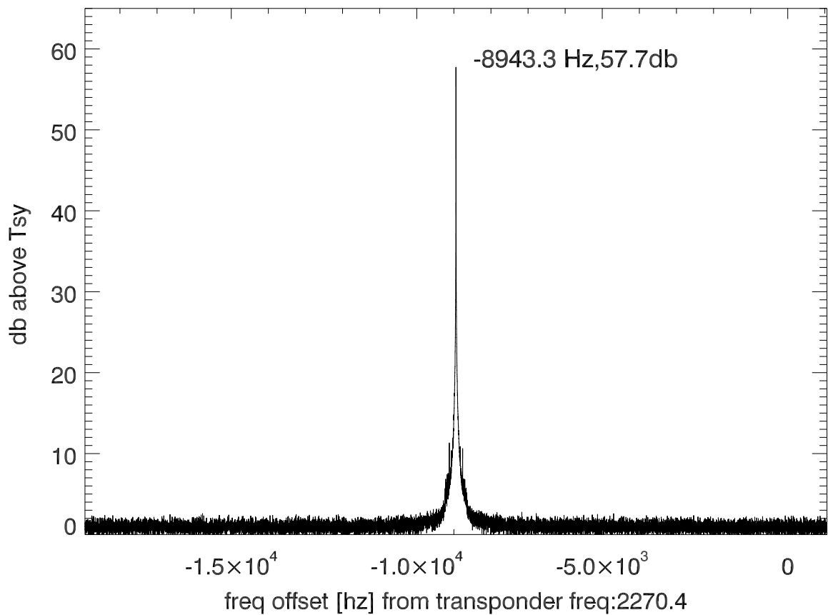
isee3 140627:180618 (UTC) spectra after doppler correction. PolB
