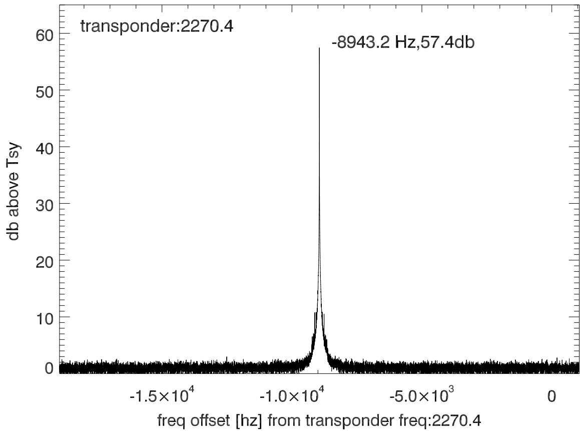
isee3 140627:180618 (UTC) spectra after doppler correction. PolA
