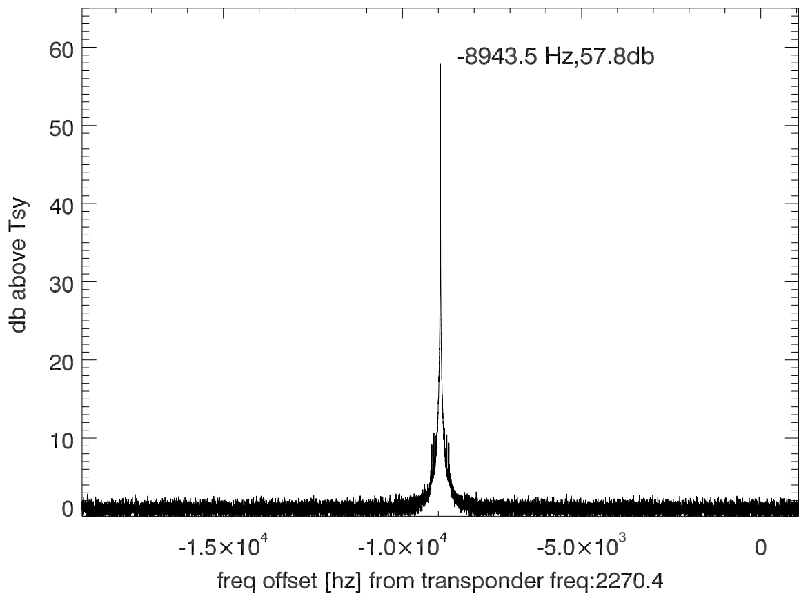
isee3 140627:180103 (UTC) spectra after doppler correction. PolB
