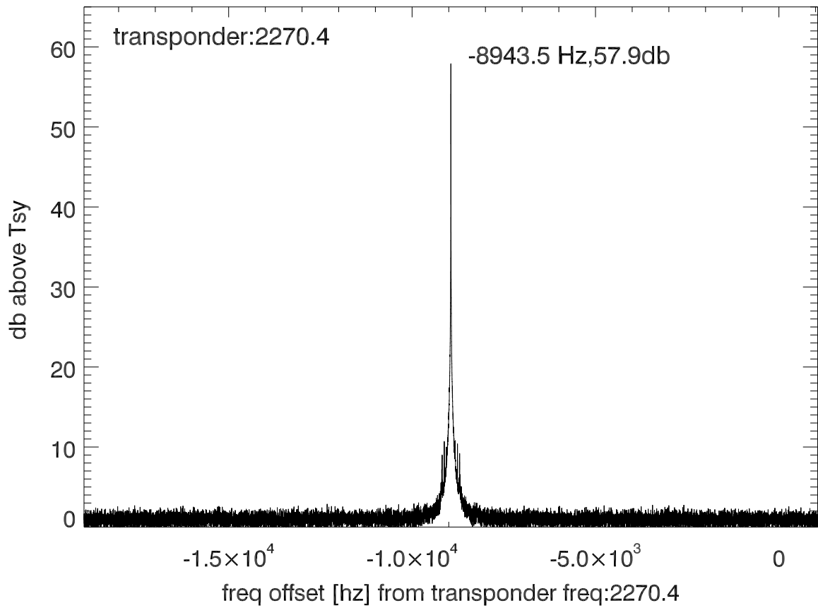
isee3 140627:180103 (UTC) spectra after doppler correction. PolA
