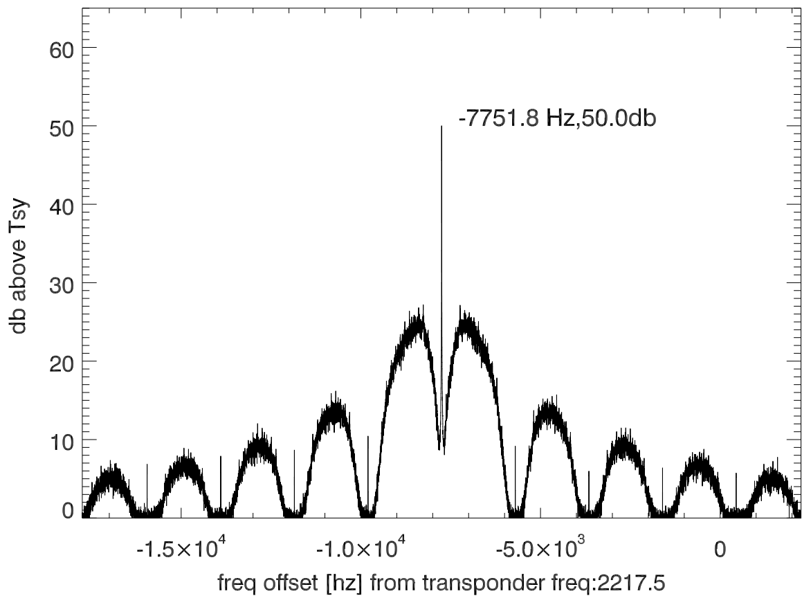
isee3 140627:195733 (UTC) spectra after doppler correction. PoIB
