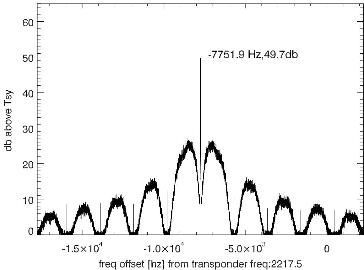
isee3 140627:195406 (UTC) spectra after doppler correction. PoIB
