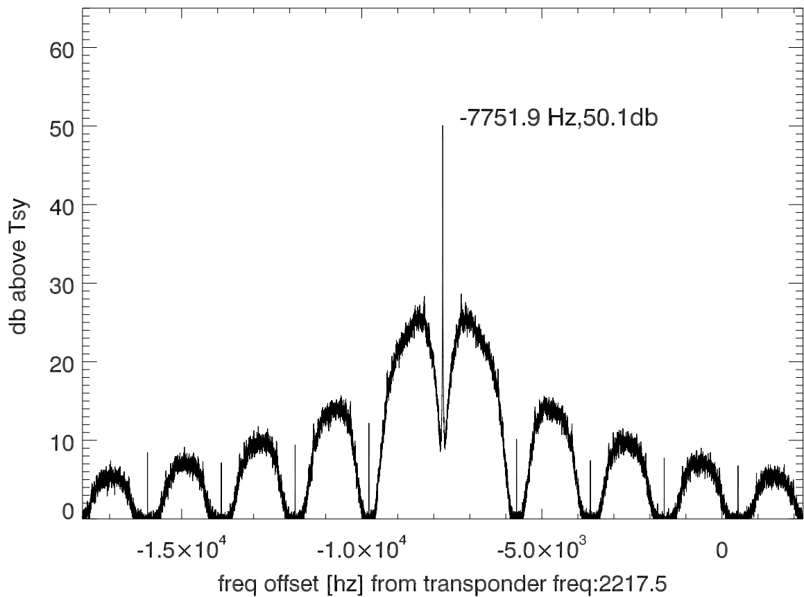
isee3 140627:195053 (UTC) spectra after doppler correction. PoIB
