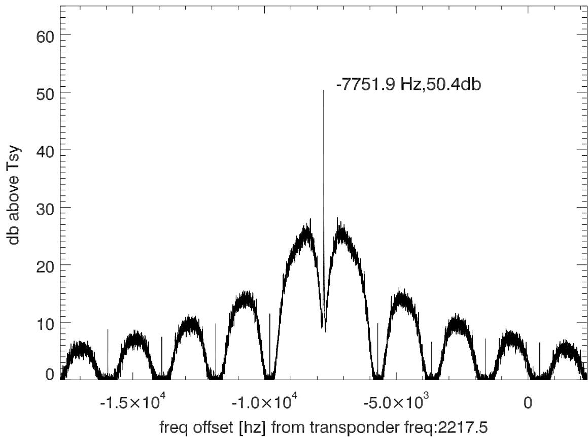
isee3 140627:194829 (UTC) spectra after doppler correction. PoIB
