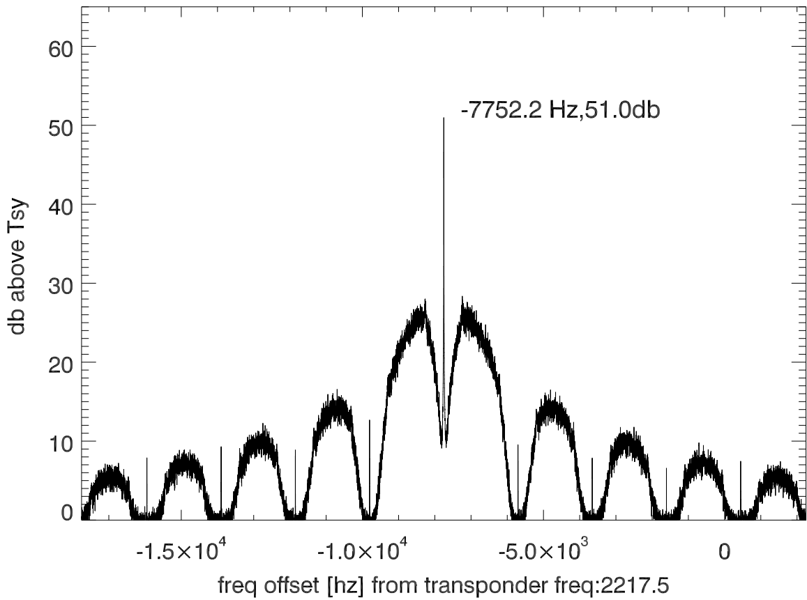
isee3 140627:194216 (UTC) spectra after doppler correction. PoIB
