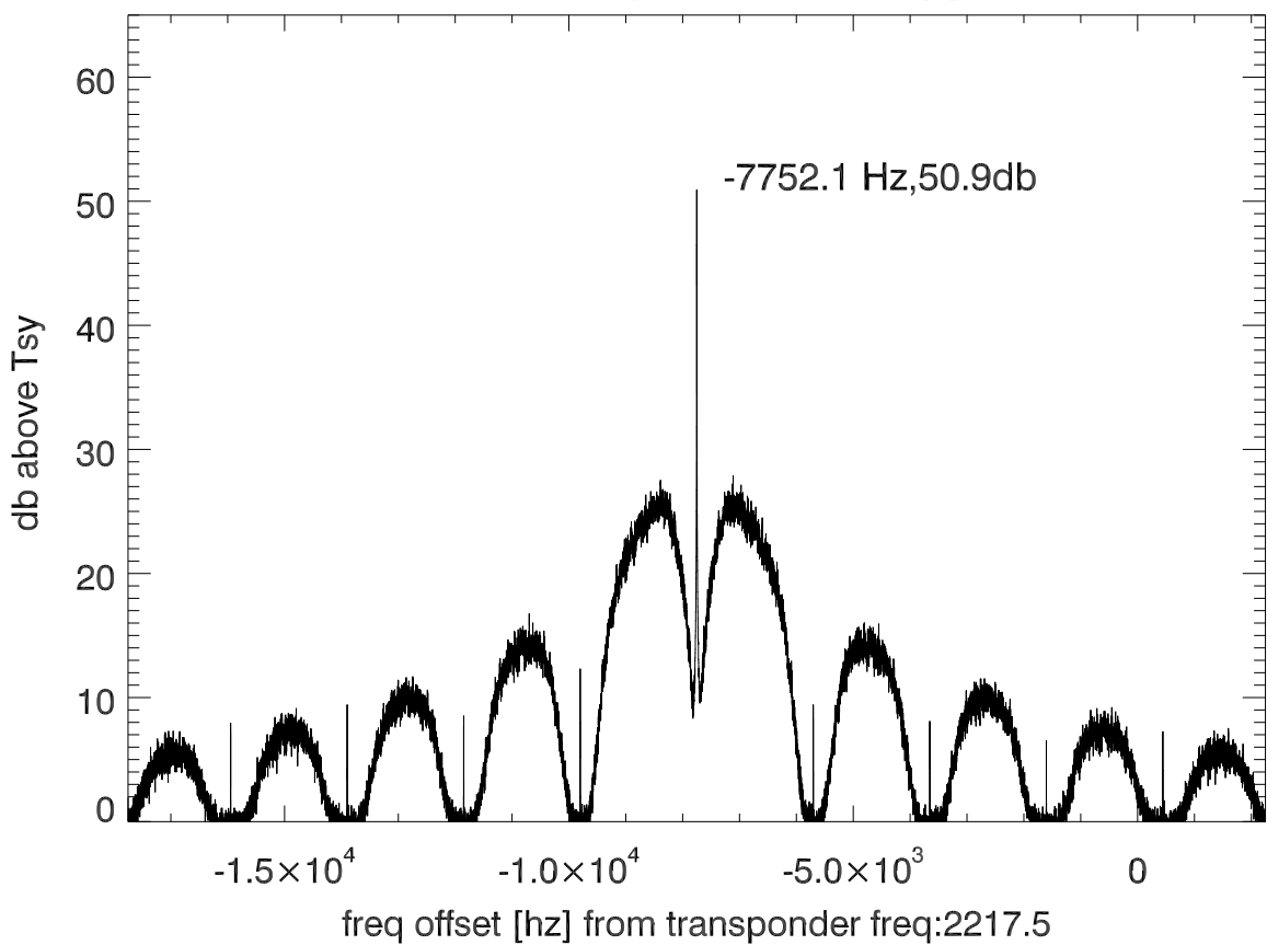
isee3 140627:193852 (UTC) spectra after doppler correction. PoIB
