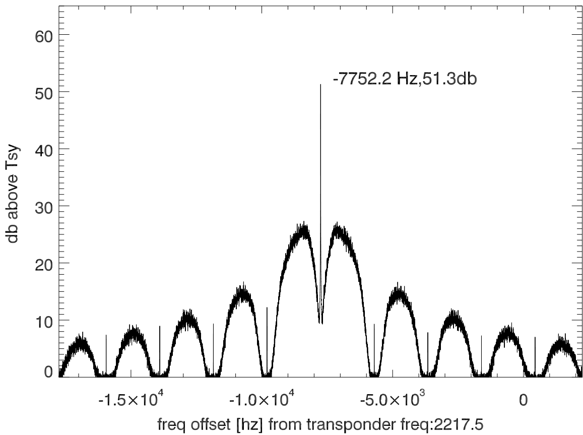
isee3 140627:193333 (UTC) spectra after doppler correction. PoIB
